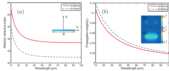
Fig. 1. (a) Effective refractive indices of GPP modes as a function of wavelength for freestanding graphene ribbons of 20 nm (the solid line) and 30 nm (the dashed line) widths. Inset illustrates a cross-section graphene nanoribbon waveguide with the width d , where the axis indicates light propagation along the z direction. (b) Propagation lengths as a function of wavelength for the freestanding graphene ribbons. Inset shows field distributions of the GPP mode at \lambda = 15 \mu\text{m} for the case of d = 30 \text{ nm} .
