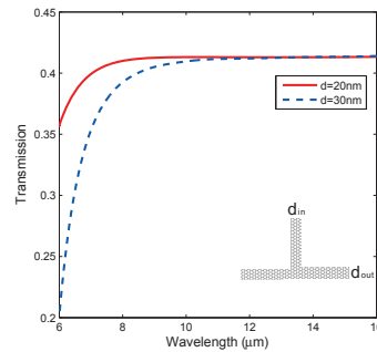
Fig. 3. Transmission spectra of graphene nanoribbon T-shape splitters (shown in the inset with the top view) for d = 20, 30 nm. In this case we choose d_{\text{in}} = d_{\text{out}} = d .
