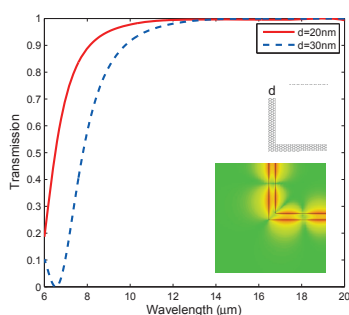
Fig. 2. Transmission spectra of graphene nanoribbon waveguide bends for d = 20, 30 \text{ nm} . Inset illustrates its top-view corresponding structure and the top-view magnetic amplitude at y = 0 when \lambda_0 = 15 \mu\text{m} and d = 30 \text{ nm} .
