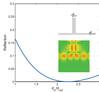
Fig. 4. Reflection coefficient of a graphene nanoribbon T-shape splitter as a function of d_{in}/d_{out} at \lambda = 12 \mu\text{m} . Inset shows its top-view corresponding structure and illustrates zero-reflection when d_{in}/d_{out} = 2.25 at \lambda = 12 \mu\text{m} .
