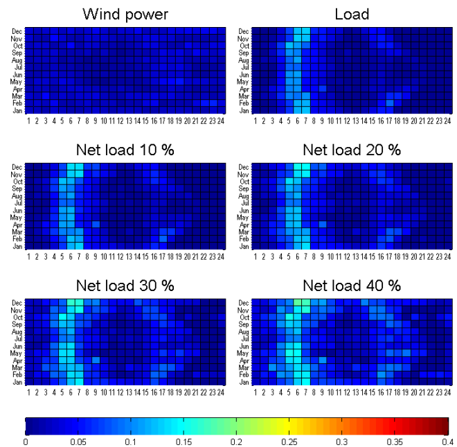
Figure 10. Timing of largest up-ramps in the Nordic region with different penetration levels, year 2011. Magnitudes of the ramps, relative to the average load, are depicted in colours (highest ramps in red).
