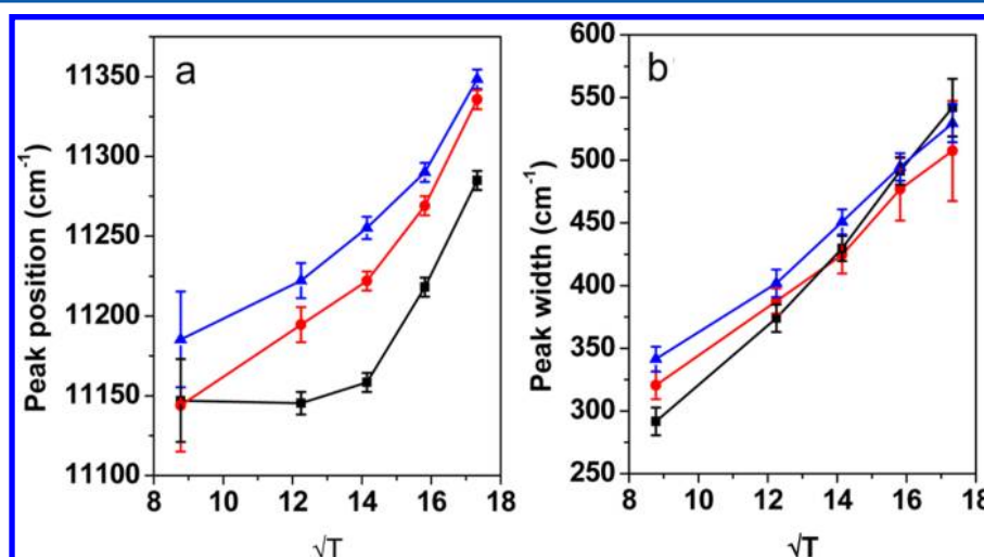
Figure 7. Temperature-dependent peak position (a) and peak width (b) for free LH2 (black), LH2-SBA-sph-1 (red), and LH2-SBA-rod (blue). The solid lines are the fits of the experimental data by a Gaussian function given in eq 1.
