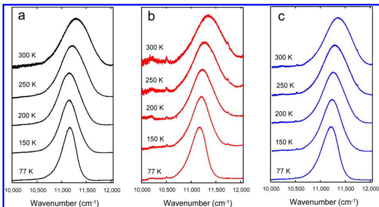
Figure 6. Temperature-dependent fluorescence emission spectra of (a) free LH2 (black curves), (b) LH2-SBA-sph-1 (red curves), and (c) LH2-SBA-rod (blue curves). The temperatures used in the measurements were in the range of 300–77 K.
