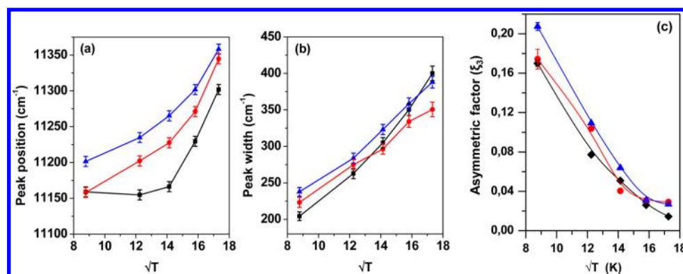
Figure 8. Temperature-dependent peak position (a), peak width (b), and asymmetric factor ( \xi_3 ) (c) for free LH2 (black), LH2-SBA-sph-1 (red), and LH2-SBA-rod (blue). The solid lines are the fits of the experimental data by the asymmetric function given in eq 6.
