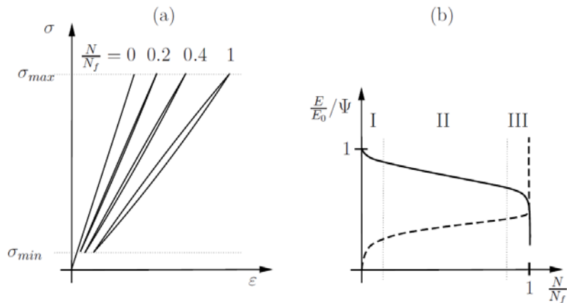
Figure 1. Sketch of a typical fatigue process observed in a glass fibre reinforced composite. (a) Stress/strain relation for a stress controlled fatigue test showing evolution of damage as function of normalised number of cycles. (b) Stiffness degradation (-) and damping propagation (--).
