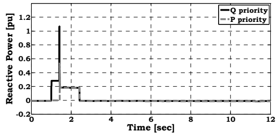
Figure 18. Reactive power response during and short after the short circuit when active or reactive power is prioritized
