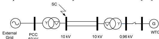
Figure 8. Single line diagram of the test system
