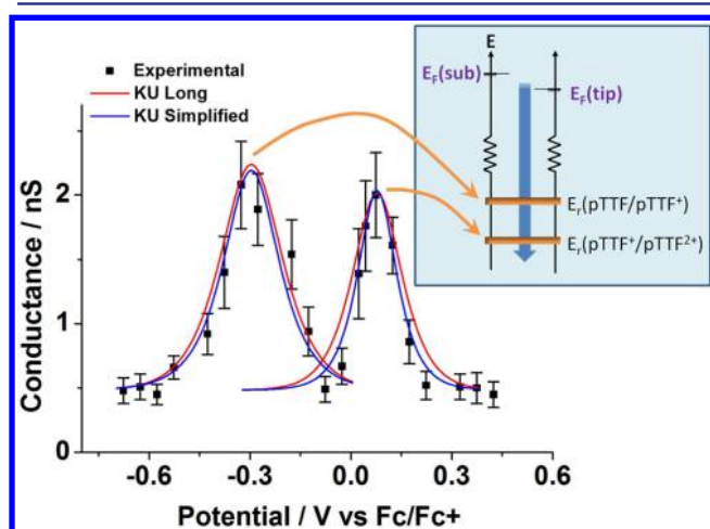
Figure 10. Conductance-sample potential relationship of 6pTTF6 in the RTIL BMOTf. The red lines show the long KU model (eq 1), and the blue lines the simplified KU model (eq 2). For both redox transitions, both KU model versions fit the experimental data well. (Inset) Schematic energy level representation of the KU model for the two redox transitions. Varying the electrode potential (represented by the bold blue arrow) changes the relative energetic positions of the tip/substrate Fermi levels and the redox levels of pTTF. However, the bias voltage between gold tip and substrate remains constant as the electrode potential is changed. As the electrode potential is scanned positive, the pTTF/pTTF + redox transition is first brought into “resonance”, and then at more positive potentials the second redox transition (pTTF 2+ /pTTF + ) comes into resonance.
