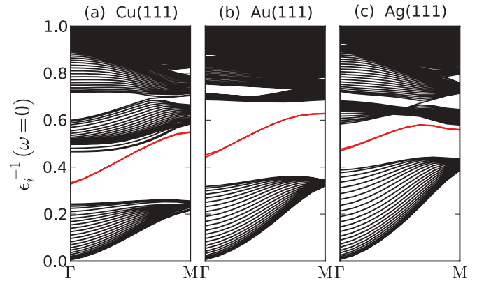
FIG. 3. (Color online) Static dielectric band structure of the (111) surfaces of Cu, Au, and Ag represented by 24 layer slabs ( \sim 5 nm thickness). \epsilon_i^{-1} are the real eigenvalues of the static inverse microscopic dielectric matrix \epsilon_{GG'}^{-1} . The bands marked in red represent the surface modes (SMs).
