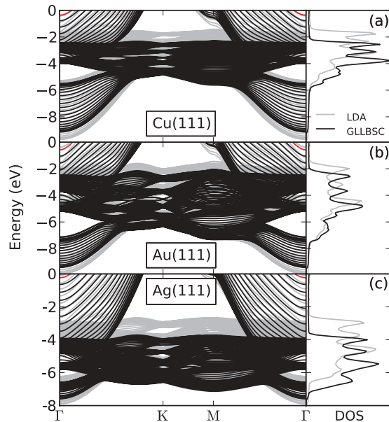
FIG. 1. (Color online) Band structure (left panel) and density of states (DOS, right panel) for the (111) surfaces, represented by 24 layer slabs ( \sim 5 nm thickness), of (a) Cu, (b) Au, and (c) Ag, calculated with LDA (gray lines) and GLLBSC (black lines). The bands marked in red represent Shockley surface states (SS). Zero energy indicates the Fermi level.
