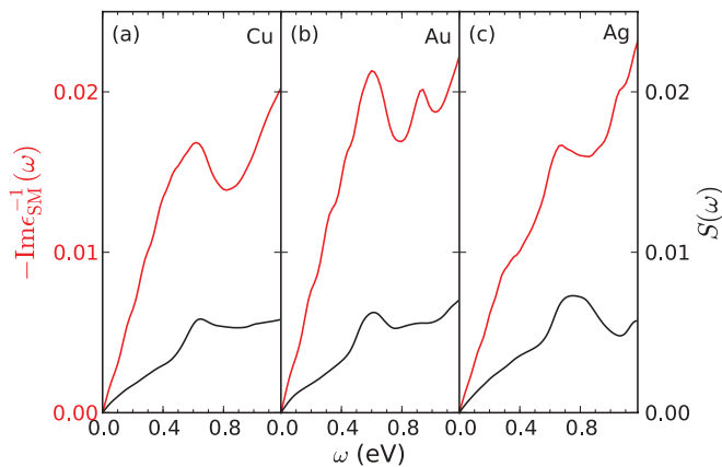
FIG. 4. (Color online) Imaginary part of the dynamic dielectric eigenvalues -\text{Im}\epsilon_i^{-1}(\mathbf{q}, \omega) for the surface states ( i = \text{SM} , red lines in Fig. 3) plotted as a function of \omega at |\mathbf{q}| = 0.125/\text{\AA} for (a) Cu(111), (b) Au(111), and (c) Ag(111), respectively. They are compared to the macroscopic loss function S(\mathbf{q}, \omega) (black lines) at the same \mathbf{q} .
