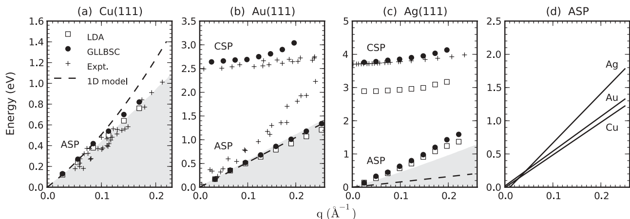
FIG. 2. Conventional and acoustic surface plasmon (CSP and ASP) dispersions for the (111) surfaces of Cu, Au, and Ag calculated with LDA (open squares) and GLLBSC (solid dots). The plasmon energies are obtained as peaks in the loss function S(\mathbf{q}, \omega) , the examples of which are shown in Fig. 4 as black lines. Previous model results (dashed line) and EELS experimental data (crosses) (Ref. 6) are shown for comparison. Shaded areas mark the Shockley electron-hole pair continuum calculated with GLLBSC. (d) Summary of the ASP dispersion obtained with the GLLBSC potential for each of the three surfaces.
