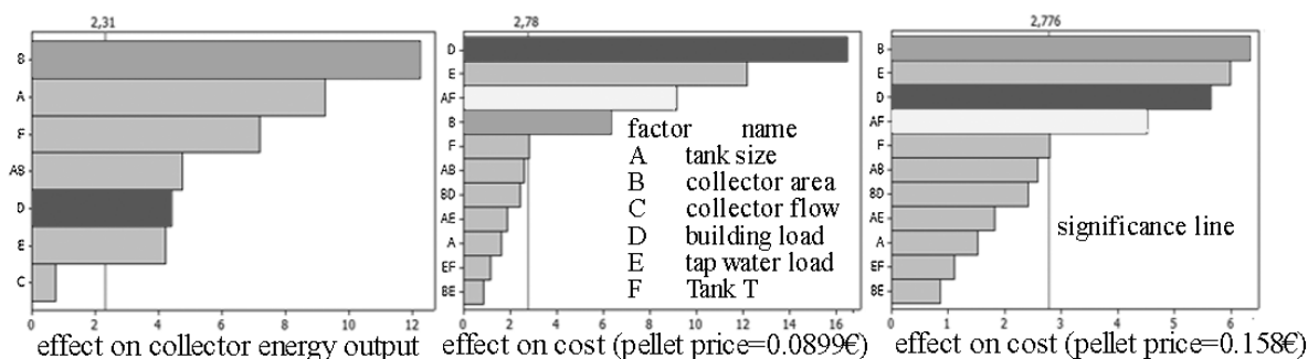
Fig. 2. Pareto plots from the initial screening. Left: collector energy output; middle: energy cost based on a low pellet price estimate; right: energy cost based on a high average pellet price estimate.
