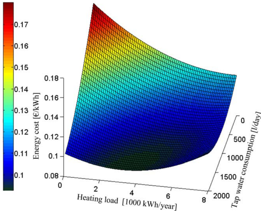
Fig 5. The energy cost in €/kWh for buildings with varying heating load and tap water consumption. The solar collector area for each building was determined by the cost-optimization in Fig 4.
