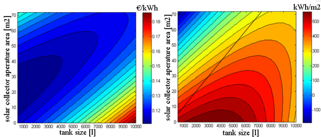
Fig. 3. Left: energy cost as a function of collector area and tank size; right: energy output as a function of collector area and tank size.
