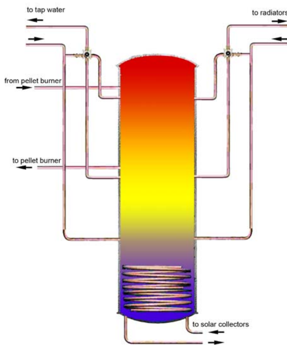
Fig. 1. Schematic of the examined system.
