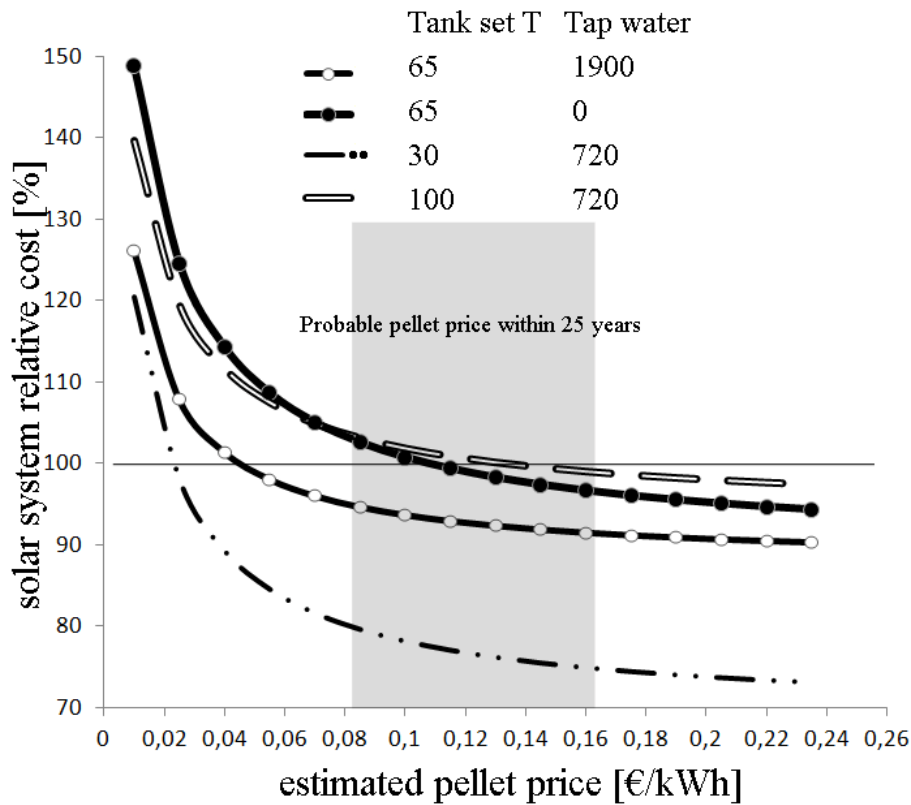
Fig. 8. Profitability of solar collector systems vs. pellet price.
