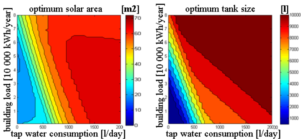
Fig. 4. Optimum for building load and tap water consumption. Left: Collector area Right: Tank size
