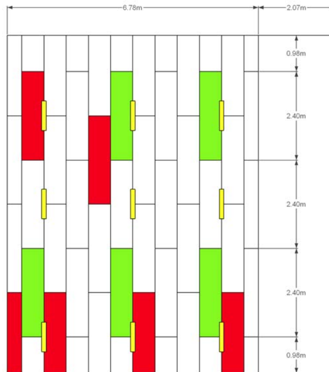
Figure 3. Placements of active cement bonded wood wool panels (red) and passive panels (white), green indicate the intended placement of the active panels.
