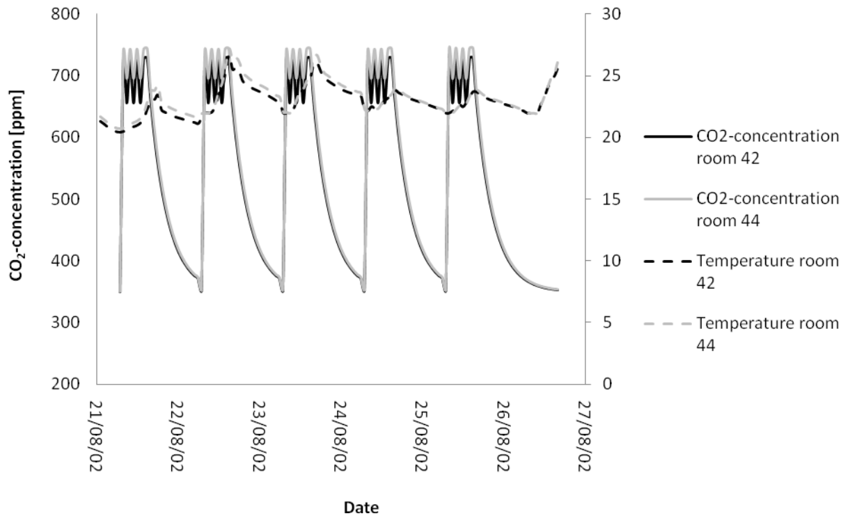
Figure 8. Simulated CO 2 -concentrations and air temperatures in the two classrooms
