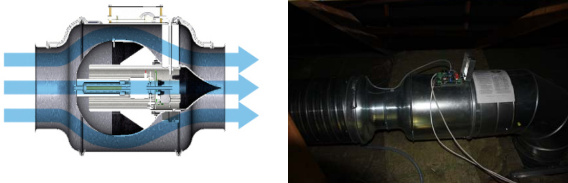
Figure 3. Principle sketch of airflow pattern in LeanVent ® dampers (left) and picture a damper installed at Vallensbæk school (right).
