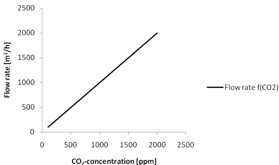
Figure 4. Theoretical ventilation flow rate to one room as a function of the CO 2 -concentration.
