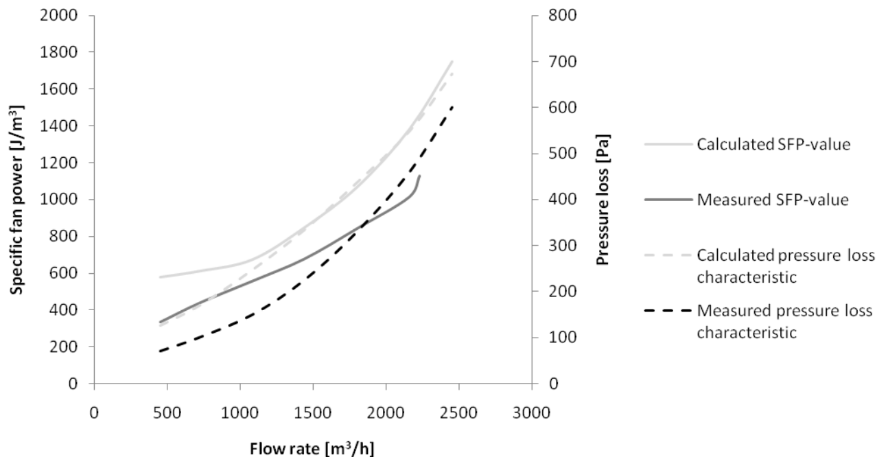
Figure 5. Calculated and measured SFP-values for the new ventilation system along the measured and calculated pressure loss Characteristics of the system.
