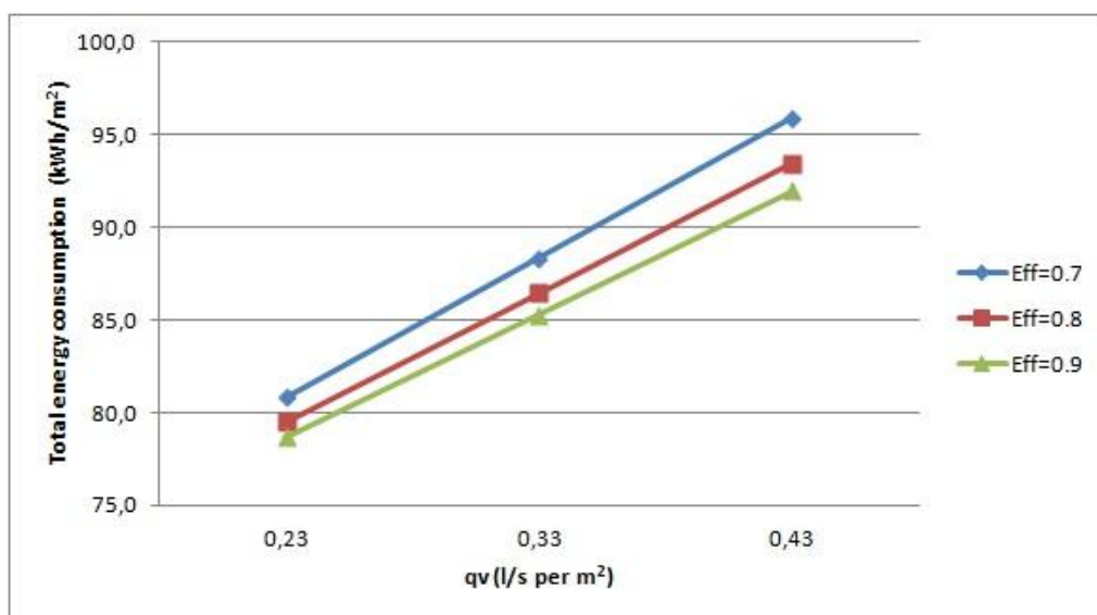
Figure 3: Sensitivity analysis of the total energy consumption with different ventilation rates (qv) and heat exchanger's efficiency (Eff).
