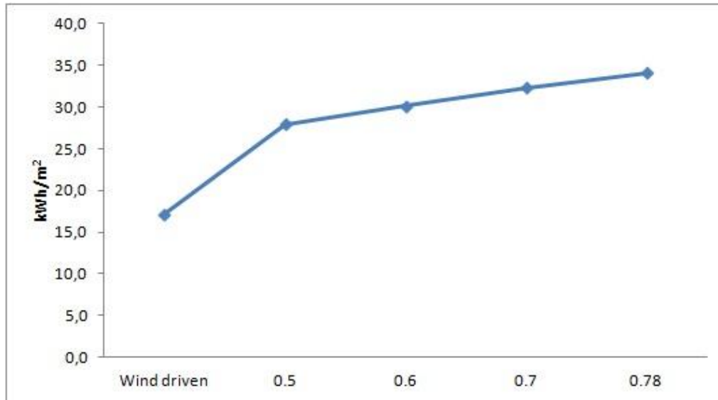
Figure 4: Energy consumption with different infiltration rates. Simulation only for March and April.
