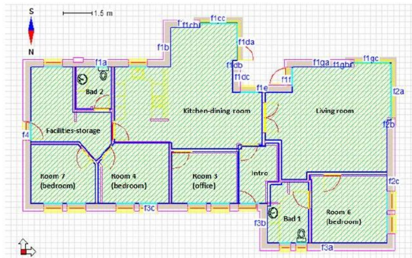
Figure 1: Layout of the house investigated with IDA-ICE 4.
