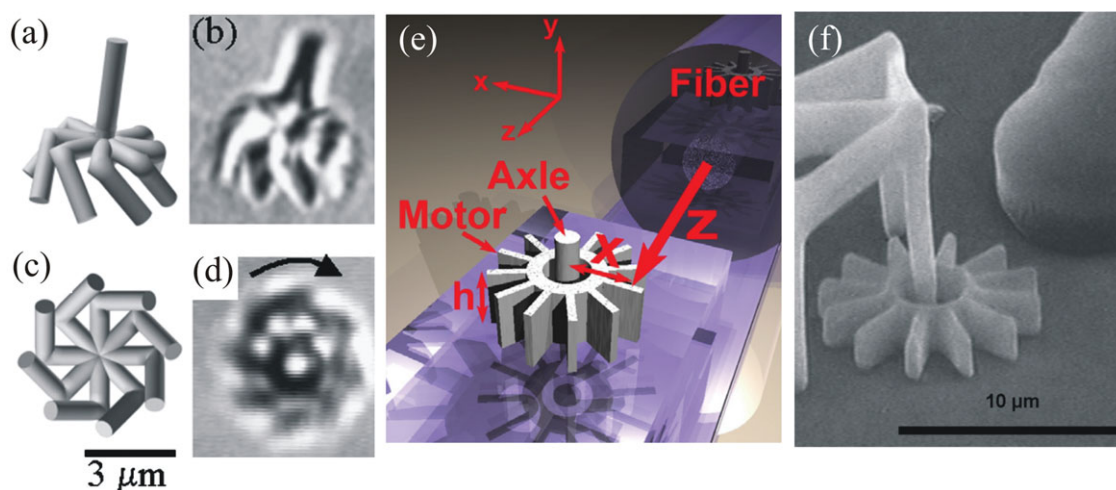
Figure 7 (online color at: www.lpr-journal.org ) System integration: the optically driven motor. (a)–(d) Free-standing micromotor rotated by a trapping beam in a microscope (graphics rendering and optical microscopy) [77]. (e) Integration using an optical fiber to supply the driving light [120]. (f) Integration where an integrated waveguide supplies the driving light [78]. (Images from respective references).
