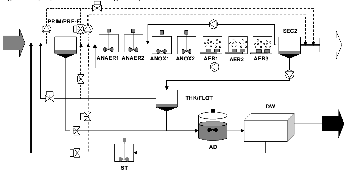
Figure 1. Plant layout of the proposed BSM2-P.
