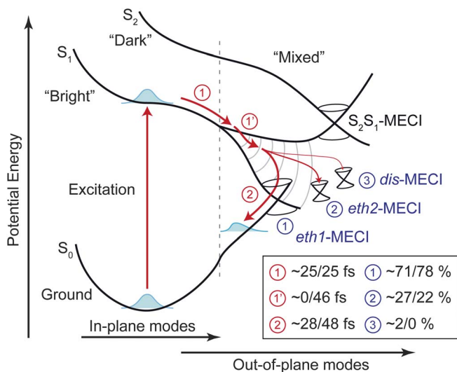
Fig. 12 Interpretation of the dynamics following excitation to S_1 with timescales and branching percentages indicated in the format CPD/Me 4 -CPD. Initially (1), nuclear motion occurs along in-plane modes such as the bond-alternation coordinate, however, for CPD motion along out-of-plane modes also takes place during this time window. Over the course of the initial nuclear motion the electronic state character mixes making an unambiguous assignment of diabatic labels to S_1 and S_2 impossible. Following the initial nuclear motion additional out-of-plane motion takes place in Me 4 -CPD (1'), which is absent in CPD, as a consequence of the slower motion of the former due to the heavy substituents. Finally (2), bifurcation on S_1 leads to a non-adiabatic transition primarily assignable to two ethylene-like MECIs.
