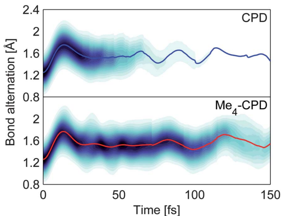
Fig. 7 Projection of the S_1 wavepacket density on the bond alternation coordinate with the expectation value indicated by the colored line for CPD (top, blue) and \text{Me}_4 -CPD (bottom, red). The bond alternation coordinate is defined as R = R_{12} + R_{34} - R_{23} with the numbering given in Fig. 1.
