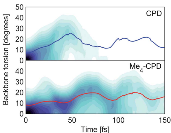
Fig. 8 Projection of the S_1 wavepacket density on the backbone torsion coordinate with the expectation value indicated by the colored line for CPD (top, blue) and \text{Me}_4 -CPD (bottom, red). The backbone torsion is the absolute value of the dihedral angle \angle C_{(1)}C_{(2)}C_{(3)}C_{(4)} , with the numbering given in Fig. 1.
