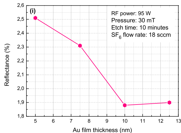
Fig. 3. Top-view SEM figures of the SiC substrates annealed at 350°C with different deposited Au film thickness and cross-sectional view SEM figures of its corresponding fabricated pseudoperiodic ARS after etching process: (a, e) 5 nm Au, (b, f) 7.5 nm Au, (c, g) 10 nm Au, and (d, h) 12.5 nm Au; (i) measured reflectance of the processed samples with different deposited Au film thickness.
