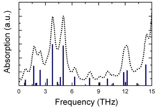
Fig. 7. Calculated absorption spectrum of 5CB (not polarization dependent). The dotted line represents a Gaussian fit.
