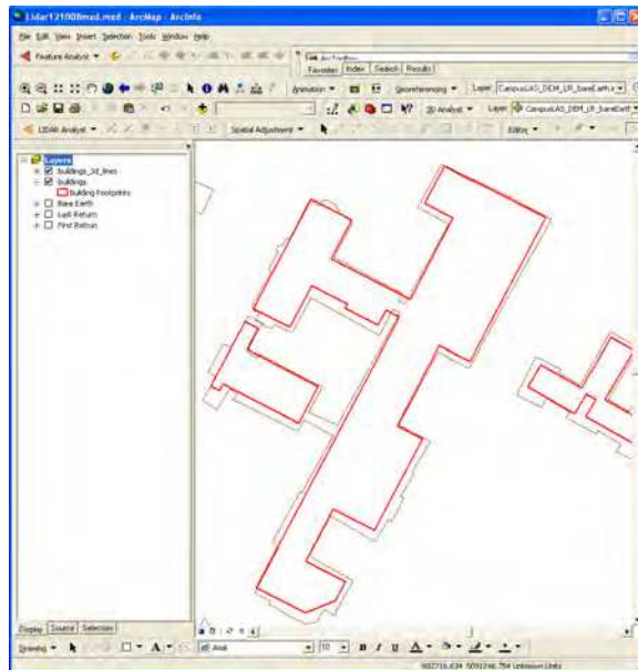
Fig. 10. Extracted building polygons (thin brown lines) compared with Cadastral buildings blueprints (thick red lines)
