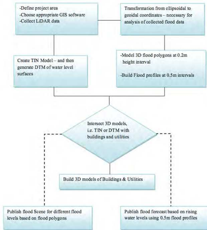
Fig. 11. The workflow of detailed methods and techniques applied for modelling of flooded buildings and infrastructure.
