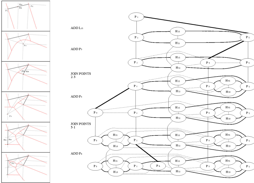
Figure 9. A sequence of map construction commands and the history of the map
