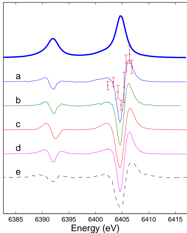
Figure 2: \text{K}\alpha spectra of the aqueous solution of (LS) [\text{Fe}(\text{bipy})_3]^{2+} (top thick blue curve, scaled down) and several HS–LS difference spectra. a : [\text{Fe}(\text{bipy})_3]^{2+} laser on – laser off transient from APS 7-ID (taken at a time delay of \Delta t = 80 ps); the circles with error bars show our previous kHz experiment at the SLS[33] for comparison. b : [\text{Fe}(\text{bipy})_3]^{2+} transient spectrum from ESRF ID26 ( \Delta t = 77 ps). c : Difference curve of the \text{K}\alpha spectra calculated with the charge transfer multiplet approach for HS and LS \text{Fe}^{2+} in \text{O}_h symmetry, from Ref. [33]. d : difference of the room temperature \text{K}\alpha spectra of the HS [\text{Fe}(\text{phen})_2(\text{NCS})_2] and the LS [\text{Fe}(\text{bipy})_3]^{2+} . e : static experiment at the thermal spin crossover of [\text{Fe}(\text{phen})_2(\text{NCS})_2] , the difference of the \text{K}\alpha spectra taken at the room temperature (HS form) and at 80 K (LS form) is shown.
