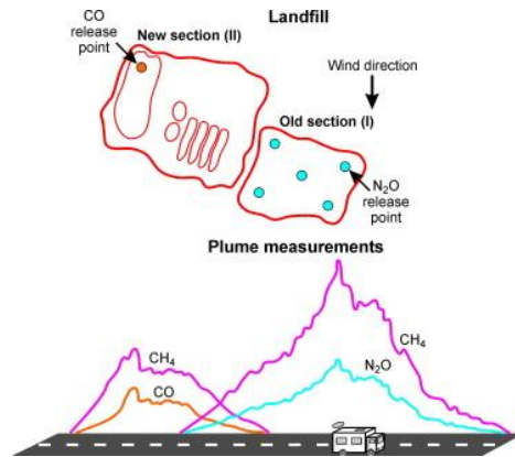
Figure 1. Dynamic plume measurements using a double tracer approach to quantify emissions from two different landfill sections (Scheutz et al., 2011).
