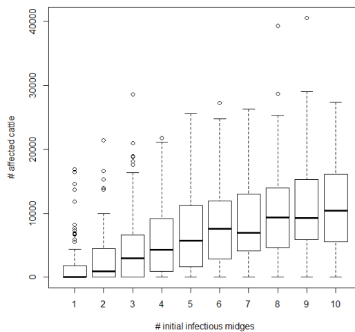
Figure 3.1: Final number of affected cattle in an epidemic as function of number of initial infectious midges arriving in southern Jutland at day 150 in 2008. 100 repetitions with the standard parameter setting. The graph indicates that there is no significant difference in median epidemic size when between 5 and 10 infectious midges initiate an epidemic.
