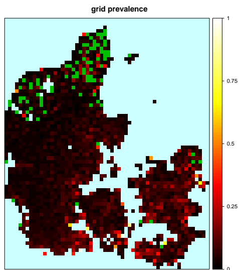
Figure 3.5: The average prevalence of SBV in the host animals per pixel, given SBV occur in this pixel (equivalent to zero prevalence being excluded when calculating average). Simulated as in figure 3.4.
