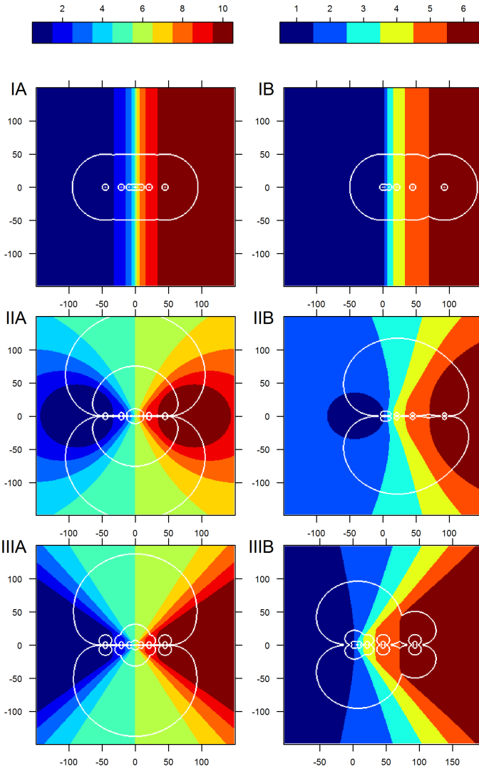
Figure D.2: Range of attraction visualization. The area of attraction for the three models. It is assumed that each trap catches a number of Culicoides proportional to the area within the range of attraction (white lines). The plots represent modeled fields of 300 by 300 meters with one transect of traps from Fig. D.1. The colors (color-key on top) indicate which trap a Culicoides in this area will end up in, with trap numbers corresponding to numbers in Fig. D.5. The white lines indicate different cutoff points in range of attraction (light intensity). These plots thereby represent the functions T^k(x, y) , where the white lines in each plot indicate the three cutoffs, I_C , also indicated in Fig. D.5, which corresponds to a range of attraction of 5 and 50 meters and the best fit. Model III is presented with \sigma = 10 . The left column is setup A, the right column is setup B. In model I (top) Culicoides always fly to the nearest trap, in model II (middle) Culicoides fly towards the area of highest light intensity, and in model III (bottom) Culicoides fly towards what they perceive as the brightest light, as illustrated in Fig. D.3.
