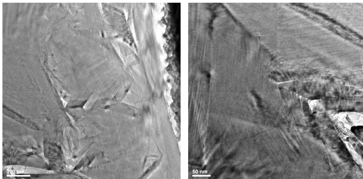
a. Dispersed batches with planar boundaries, assumed to be twin boundaries.
