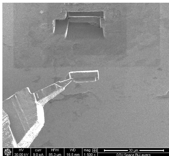
c) Sample, attached to the Omniprobe, lifted out of the bulk material
