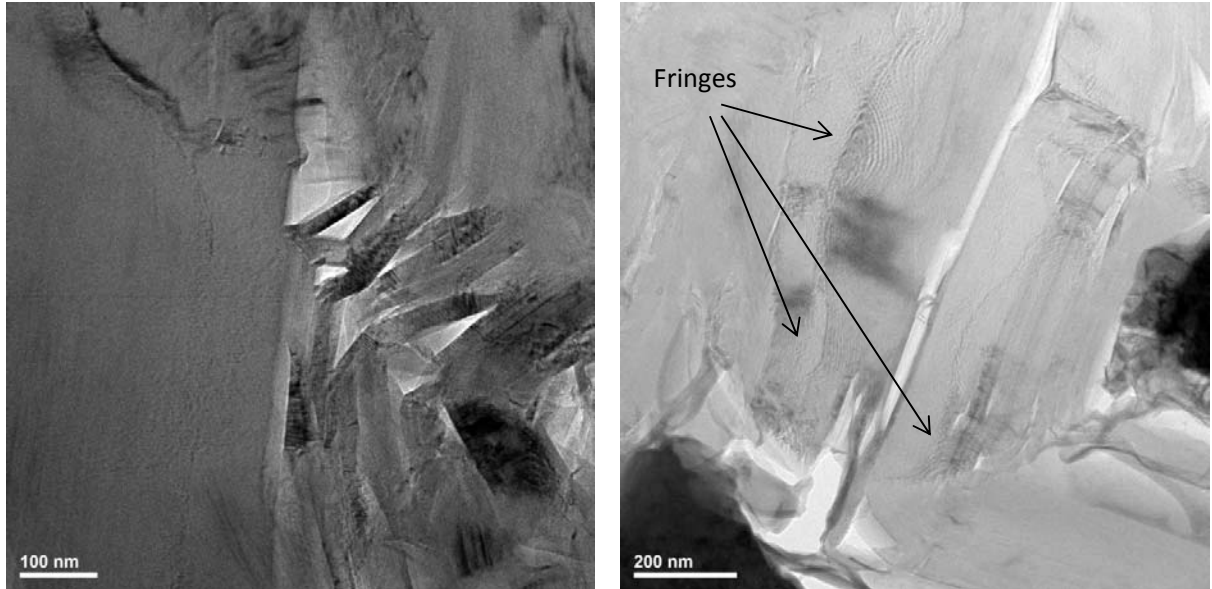
a. Twisted platelets of graphite along the twin-boundary
