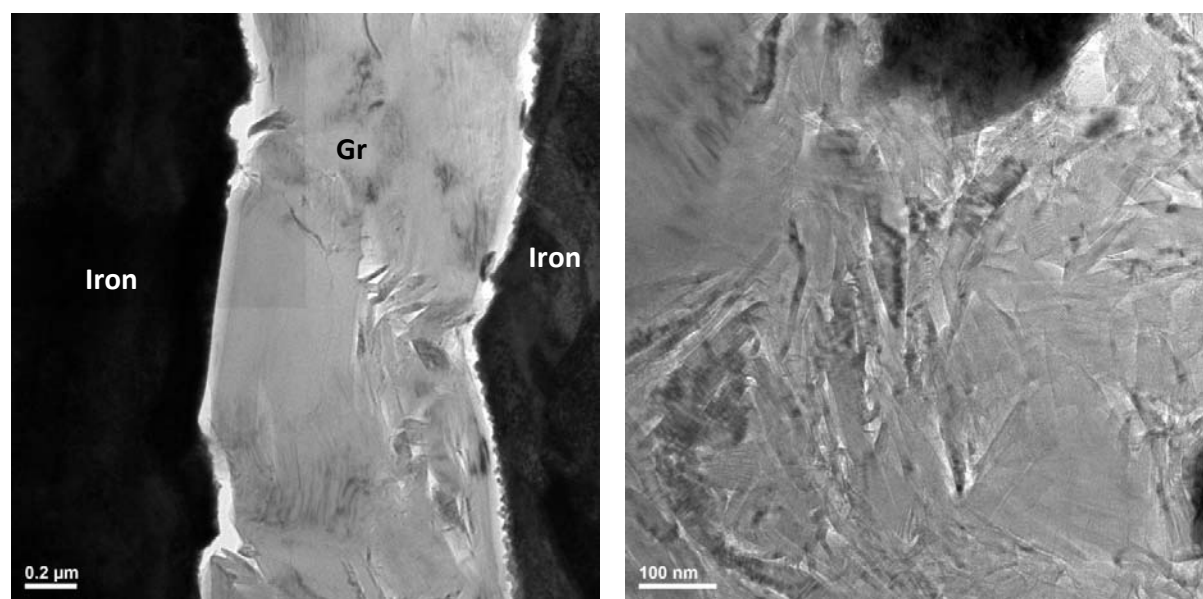
a. The middle region of the lamella, twisted platelets of graphite along the central region.
