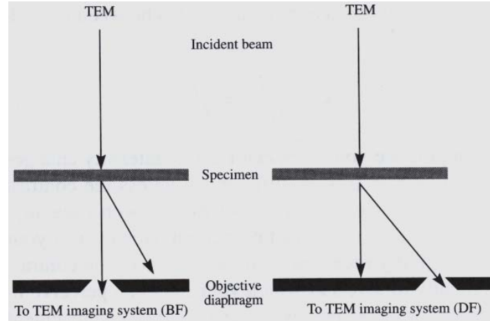
Fig. 2. BF and DF imaging on TEM
