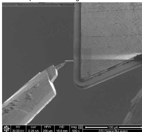
d) The Omniprobe/sample assembly positioned onto a grid
