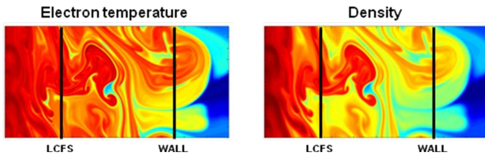
Figure 2. High resolution (2048x1024) ESEL simulation showing snapshots of the electron temperature (left) and density (right). Color scales are logarithmic to enhance the dynamics in the SOL and wall regions.
