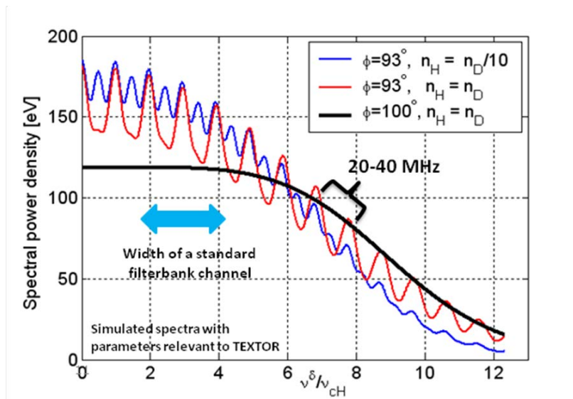
Figure 7. Simulated spectra illustrating the sensitivity of the ion cyclotron structure in CTS spectra to plasma composition and to the resolved angle, \Phi = \angle(k^\delta, B) , between the magnetic field and resolved fluctuation wave vector. The frequency scale is normalized by the hydrogen ion cyclotron frequency, and the ion cyclotron structure shows up as peaks form peaks separated roughly by the cyclotron frequency of the most common ion species in the plasma – which is well below the frequency resolution of the filter bank used for fast-ion measurements.
