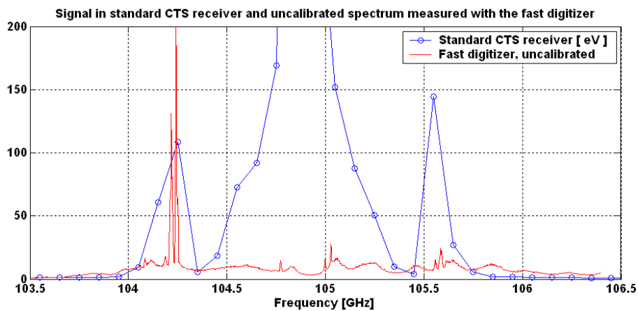
Figure 23. A comparison of measurements with the standard CTS receiver setup used for fast-ion measurements and uncalibrated measurements with the new setup for high-resolution measurements. The secondary emission was seen right after the neutral beam injector was turned on as broad peaks at frequencies around 104.3 and 105.6 GHz. With the new digitizer these peaks can be resolved in detail and are found to consist of several discrete peaks with frequency intervals around 23 MHz (i.e. in the ion cyclotron range of frequencies for these plasmas).
