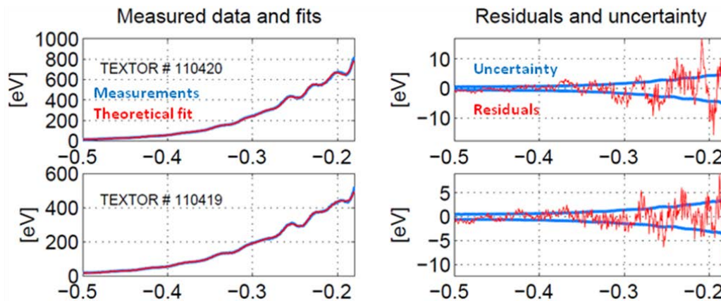
Figure 8. Left: measured spectra and theoretical fits for two discharges at TEXTOR for which the CTS spectrum contains ion cyclotron structures. Right: Residual in the fits compared to the measurement uncertainties for the same discharges.
