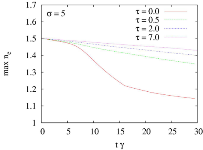
Figure 3. Maximal blob particle density as a function of time for blobs having widths 5\rho(\tau=1) , for different ion to electron temperature ratios \tau .
