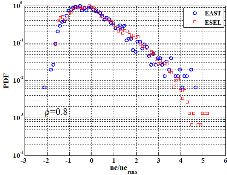
Figure 4. Comparison of the PDF of density fluctuation signal from experiment and simulation results at the radial position \rho=0.8 . Here, \rho denotes the radial position normalized by the SOL width.
