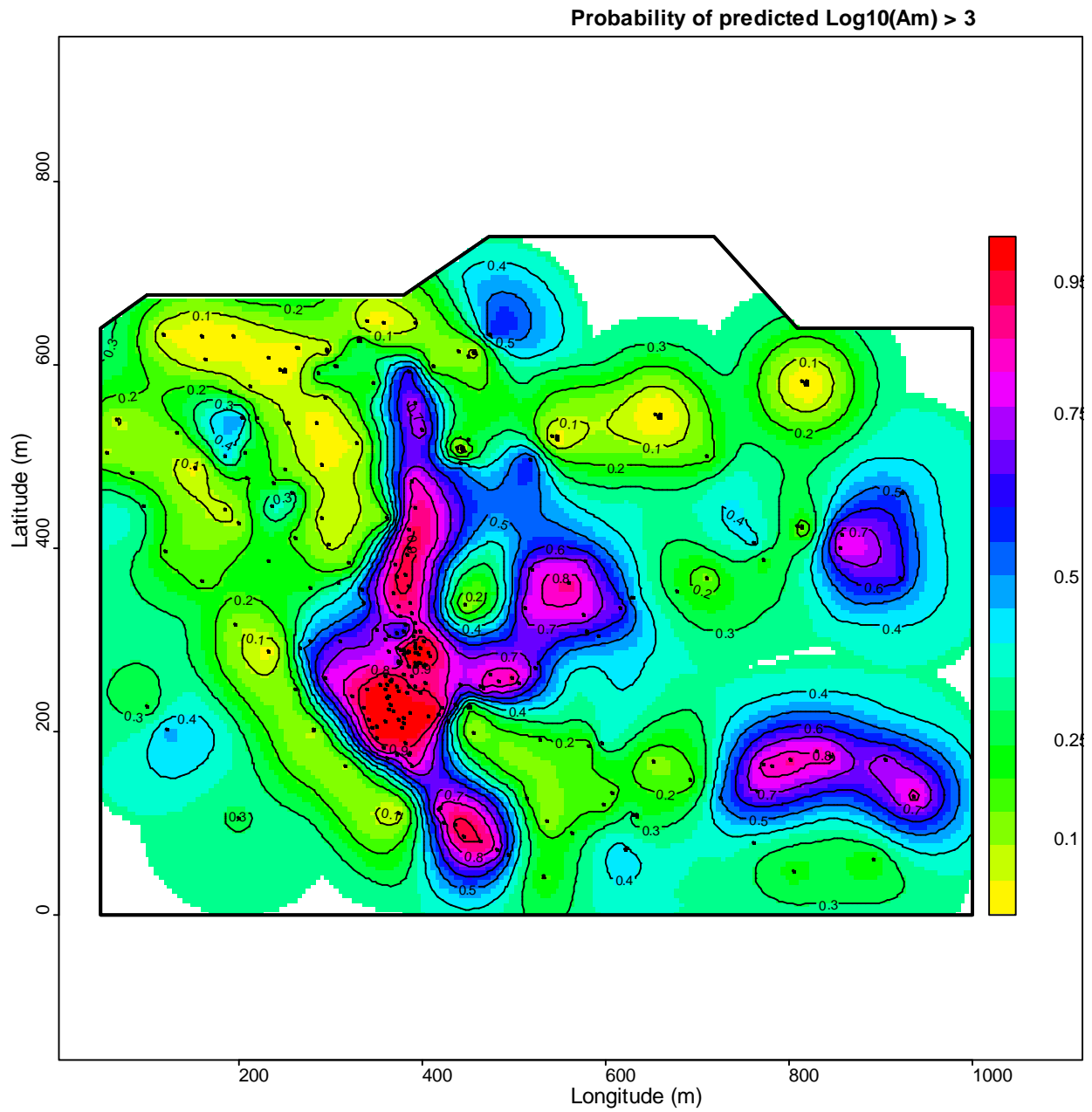
Figure 35 Probability of the \text{log}_{10} concentration exceeding 3
