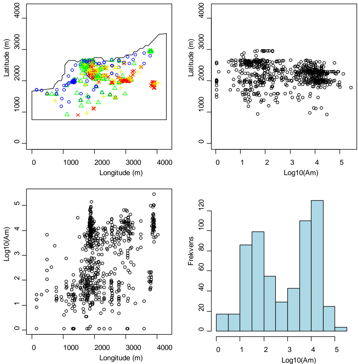
Figure 18 Summary plot of the \log_{10}(^{241}\text{Am}) data in region 2. In the upper left: Blue circle is the 0-25% quantiles, green triangle is the 25-50% quantiles, yellow plus is the 50-75% quantiles and red cross is the 75-100% quantiles.
