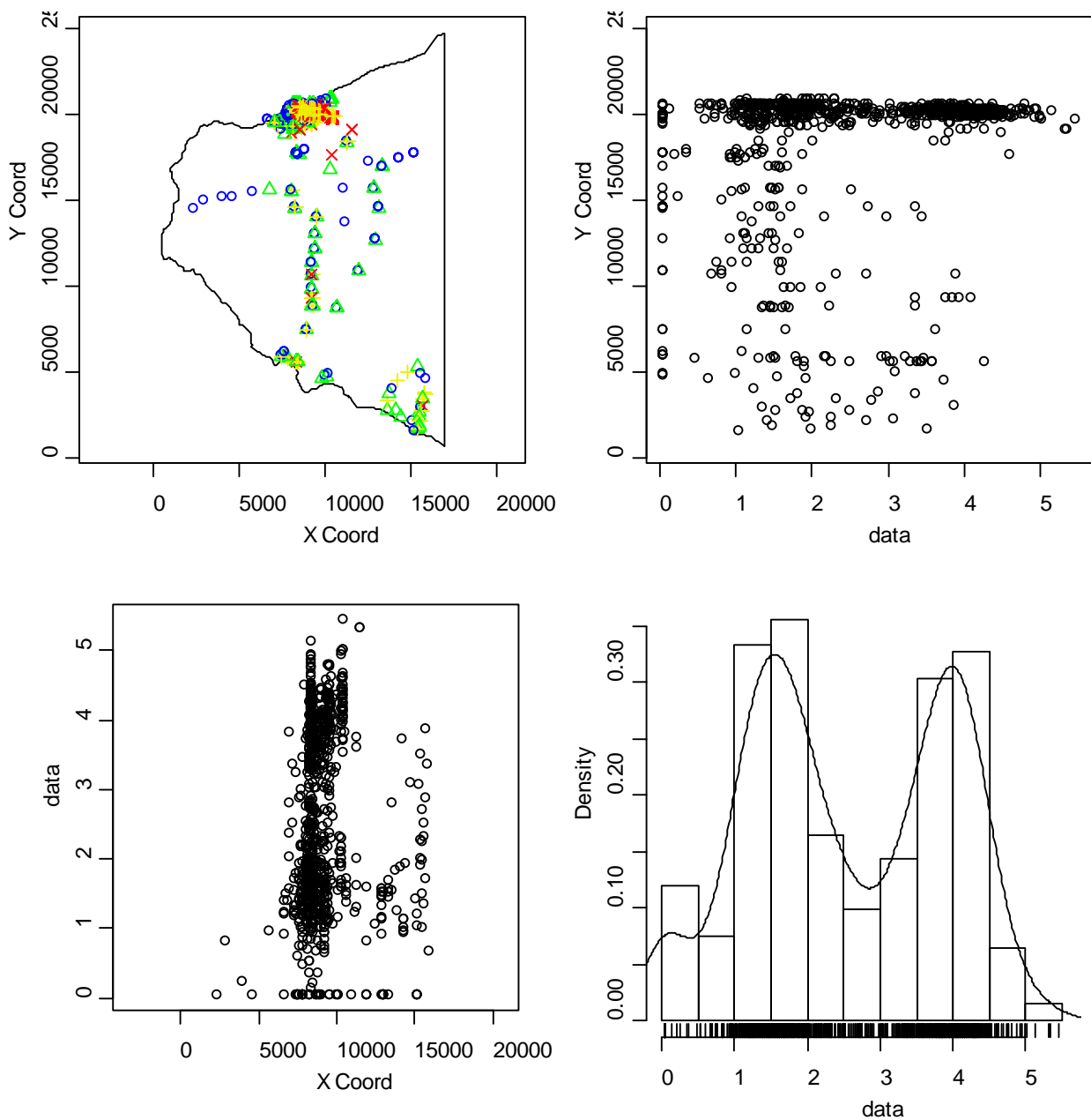
Figure 8 Summary plot of the \log_{10}({}^{241}\text{Am}) data in region 1. Upper left: Blue circle is the 0-25% quantiles, green triangle is the 25-50% quantiles, yellow plus is the 50-75% quantiles and red cross is the 75-100% quantiles.
