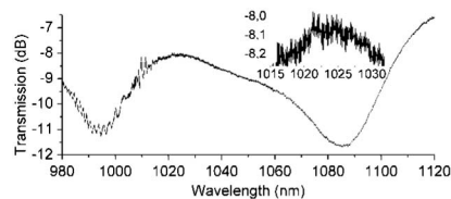
Fig. 5. MPI measurement of a GVD compensating PM HOM module with a resolution of 0.1 nm. The MPI and 1 dB bandwidth of the module are determined to -39.7 dB and 41 nm, respectively. The inset shows the basis of the MPI calculation.
