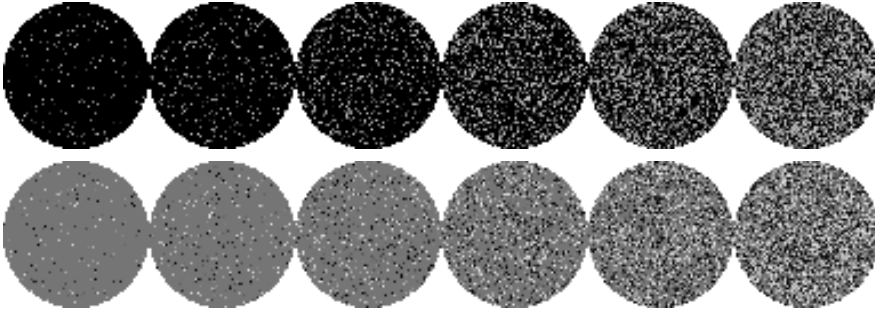
FIG. 3.2. Sparse phantom image instances of class spikes (1st row, black is 0, white is 1), and of class signedspikes (2nd row, black is -1 , white is 1). Relative sparsity from left to right is \kappa = 0.05, 0.10, 0.20, 0.40, 0.60, 0.80 .
