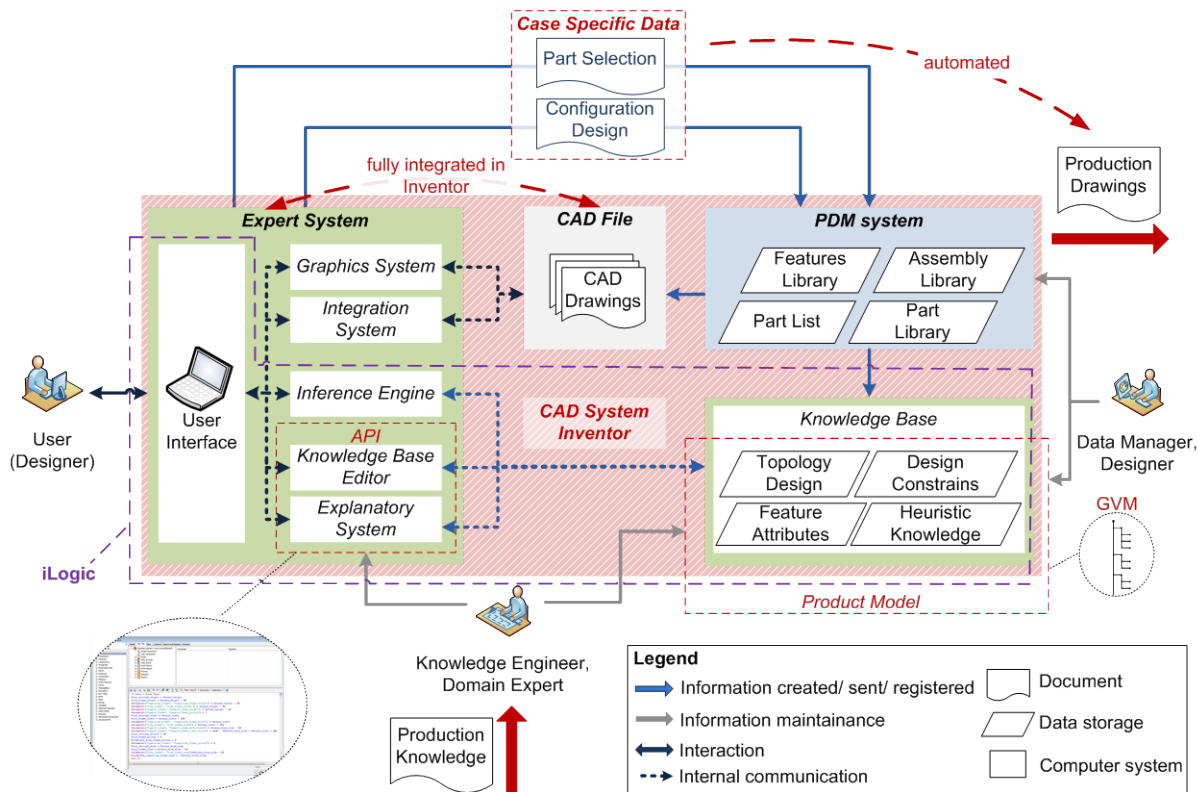
Figure 1 Integrated system architecture for automated precast design
