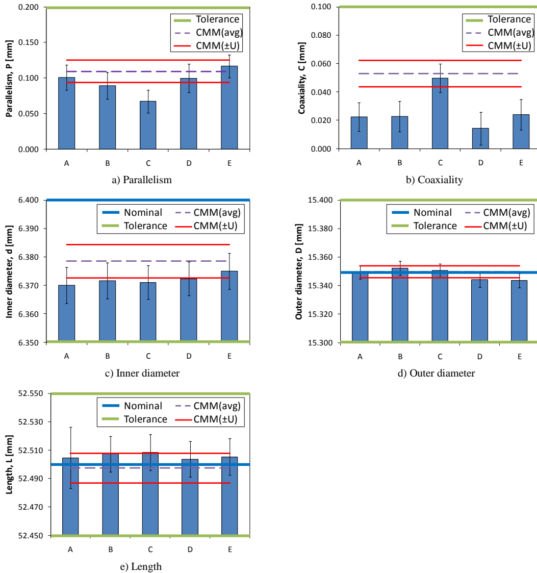
Fig. 4. Results of geometrical and dimensional tolerance analysis. Each column represents an average value of three reproduced CT measurements. The error bars represent expanded uncertainty for CT measurements at 95% confidence interval. The designation of symbols A–E is explained in Fig. 3 and refers to a combination of variables employed. The violet dashed lines are average values measured by the CMM on 16 randomly chosen parts from a production batch, and the red full lines show the range of expanded uncertainties at 95% confidence interval.
