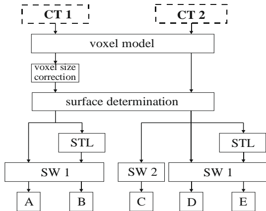
Fig. 3. Measuring procedure for data evaluation
