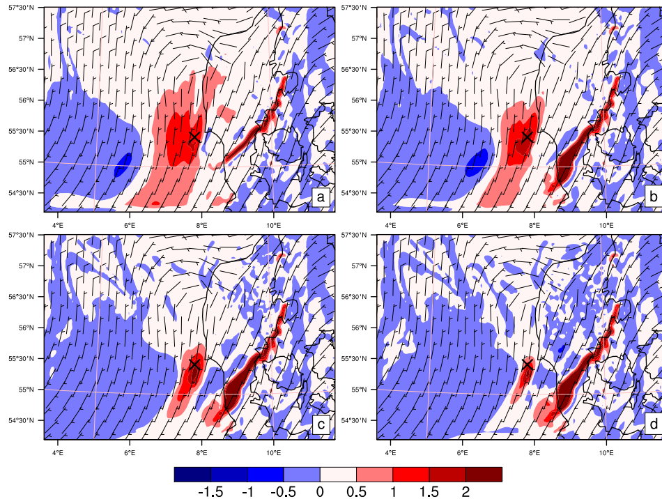
Figure 6.13: Wind speed increments in \text{ms}^{-1} at the second model level ( \sim 46 m agl) for the assimilation of nacelle winds at the location of the wind farm Horns Rev I (denoted by the cross) for a radius of influence of (a) 120 km, (b) 80 km, (c) 40 km and (d) 20 km after 6 hours of nudging. The wind barbs are taken from the original forecast (first guess).
