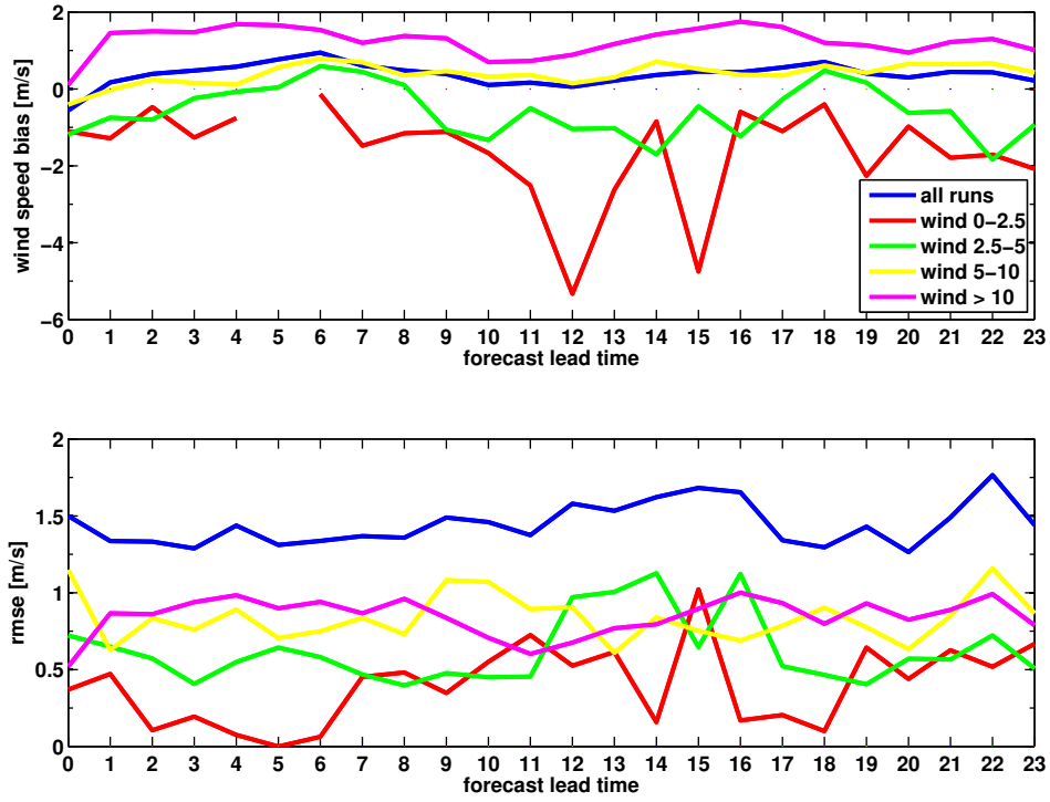
Figure 3.3: Wind speed biases (upper panel) and RMSE (lower panel) in \text{m s}^{-1} for Høvsøre for forecast lead times from 0 (analysis) to +23 hours for wind speed bins of 0-2.5 \text{ m s}^{-1} , 2.5-5 \text{ m s}^{-1} , 5-10 \text{ m s}^{-1} and >10 \text{ m s}^{-1} for the runs initialized at 00 and 12 UTC combined. The blue line depicts the bias and RMSE for all the simulations.
