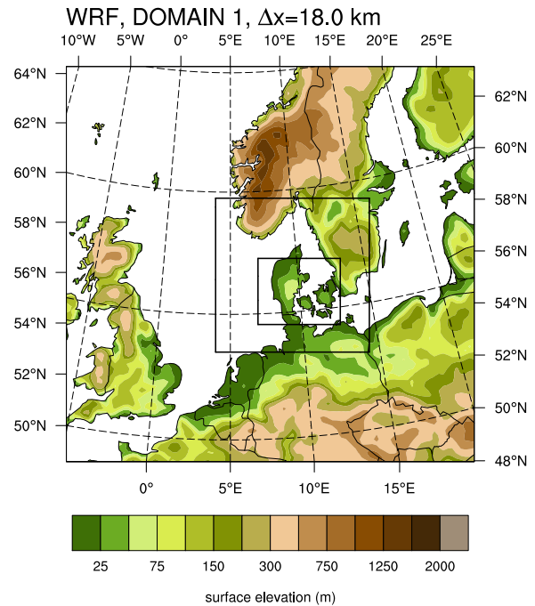
Figure 3.5: Domain configuration and terrain elevation of the WRF model setup. The black squares indicate the boundaries of two nested domains.
