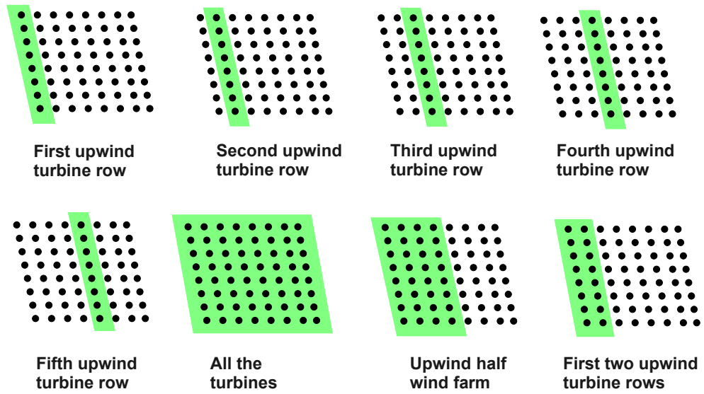
Figure 6.5: Schematic for the different grouping strategies of nacelle winds. Black dots represent the turbines, underlaid is the number of turbines used to calculate the median.
