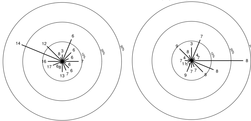
Figure 3.13: Wind roses for 60 m wind observations at Høvsøre during the periods: (left) 1–14 October and (right) 15–30 October 2009. The mean wind speed for each wind direction is given.
