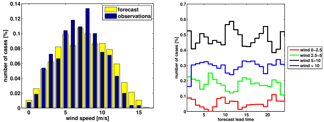
Figure 3.4: Left: Histogram of forecast (yellow) and observed wind speeds (blue). Right: Distribution of the different wind speed classes for each forecast hour.
