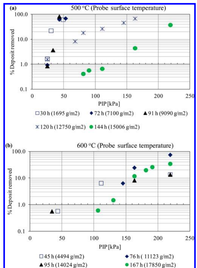
Figure 11. Percentage of deposits removed as a function of applied peak impact pressure (PIP) at different probe exposure times and deposit mass loads: (a) probe surface temperature = 500 \text{ }^\circ\text{C} ; (b) probe surface temperature = 600 \text{ }^\circ\text{C} .
