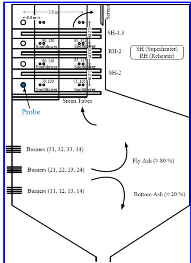
Figure 1. Schematic drawing of the AMV1 boiler outlining the position of the plant sootblowing near the experimental setup. In total, 12 sootblowers affect the deposit shedding process, 6 along the left wall of the boiler and 6 along the right wall of the boiler. The distance of each sootblower from the probe measuring position is also shown. Sootblower 70 was very near the probe measuring position (1 m to the left) and was shut down during tests 1–5. The first number in a pair of two numbers shows the sootblowers located on the same wall where the probe is located (left wall, burner location), whereas the second number shows the sootblowers located on the opposite wall (right wall, burner location).
