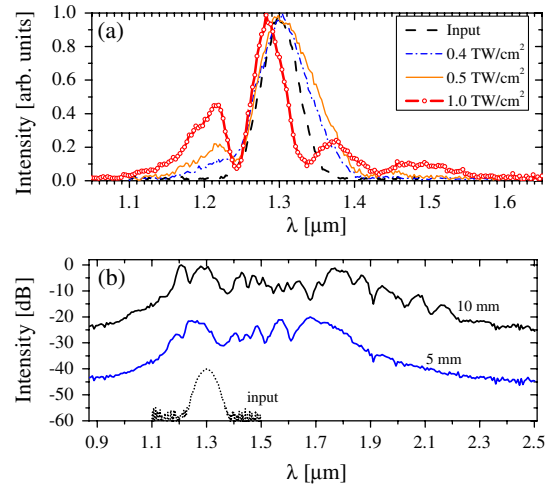
FIG. 2 (color online). (a) Spectra after a 1 mm LN crystal for various input intensities. (b) Spectra after 5 and 10 mm propagation using I_{\text{in}} = 1.0 \text{ TW}/\text{cm}^2 (averaged over 1100 shots). The spectra in (b) are offset 20 dB from each other for clarity.
