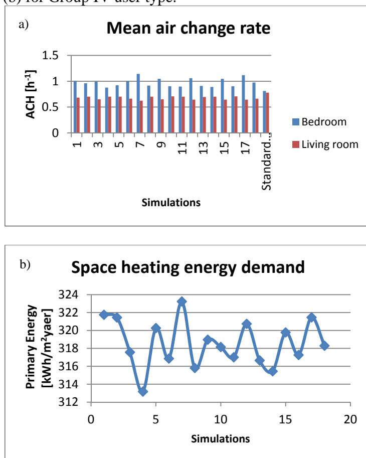
Figure 1. Distribution of mean air change rate (a) and space heating energy demand (b) for Group IV user type.
