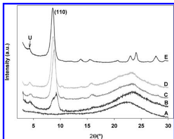
Figure 7. X-ray diffraction patterns of (A) neat rye arabinosylin (RAX), (E) sepiolite and composite films of RAX-sepiolite, RAX-sepiolite (B) 97.5:2.5, (C) 95:5, and (D) 90:10. (110) indicates the position of the characteristic peak from sepiolite and U an unidentified mineral in the sepiolite sample.
