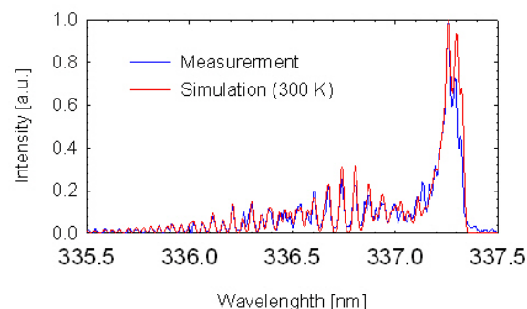
Figure 1. Measurement and simulation for the 0-0 transition of the 2 nd positive system of nitrogen in the OES of the helium DBD with ultrasonic irradiation. The best fit was found for a rotational temperature of 300 K. The measured spectral resolution (FWHM) is 20 pm.
