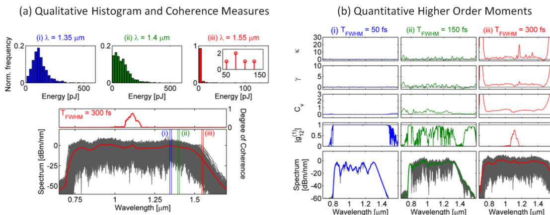
Fig 1: (a) Spectra, and calculated coherence function and histograms for a 300 fs pulse. The energy fluctuation histograms are calculated in the 10 nm windows marked in the spectrum. The inset in (iii) shows a close-up of single high energy pulses. (b) Spectra and coherence ( \log^{(1)}(g_{12}^{(2)}) ), coefficient of variation ( C_v ), skewness ( \gamma ) and kurtosis ( \kappa ) for pulse widths of 50, 150 and 300 fs.
