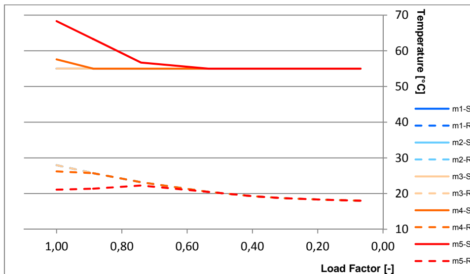
Fig. 2. The supply and return temperature profiles obtained in each mass flow limit, for the future heat demand situation
