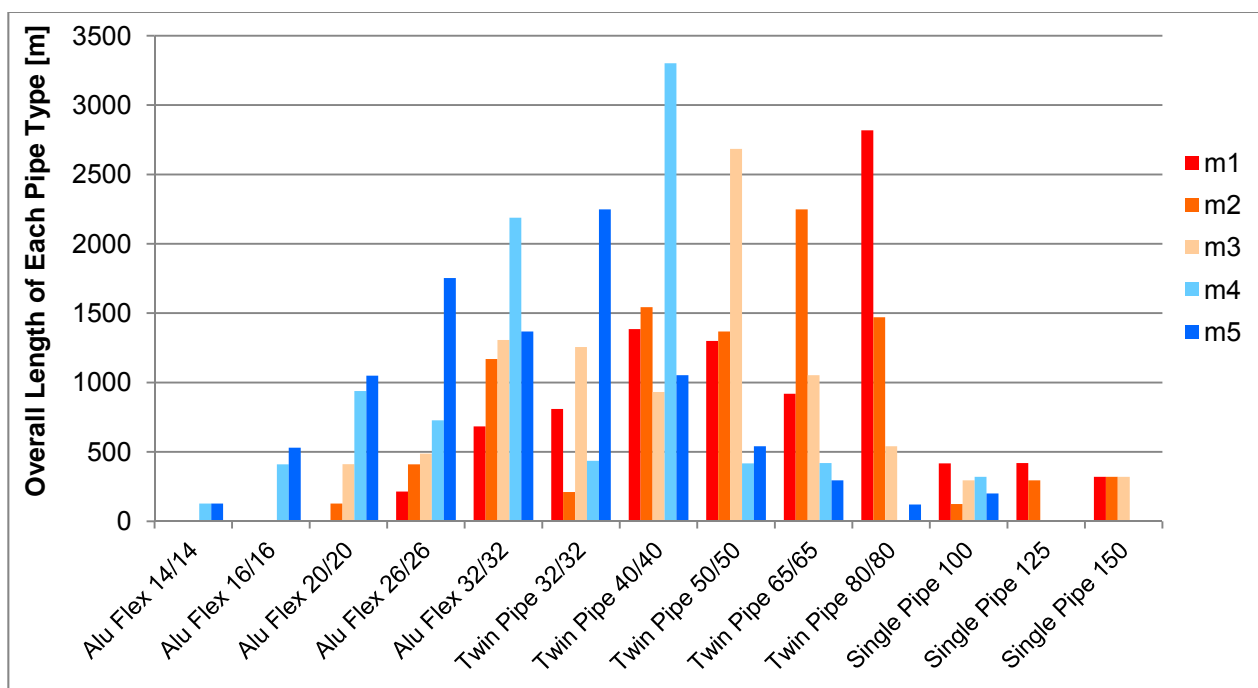
Fig. 3. The overall length of pipe diameters obtained as a result of optimization for each mass flow level
