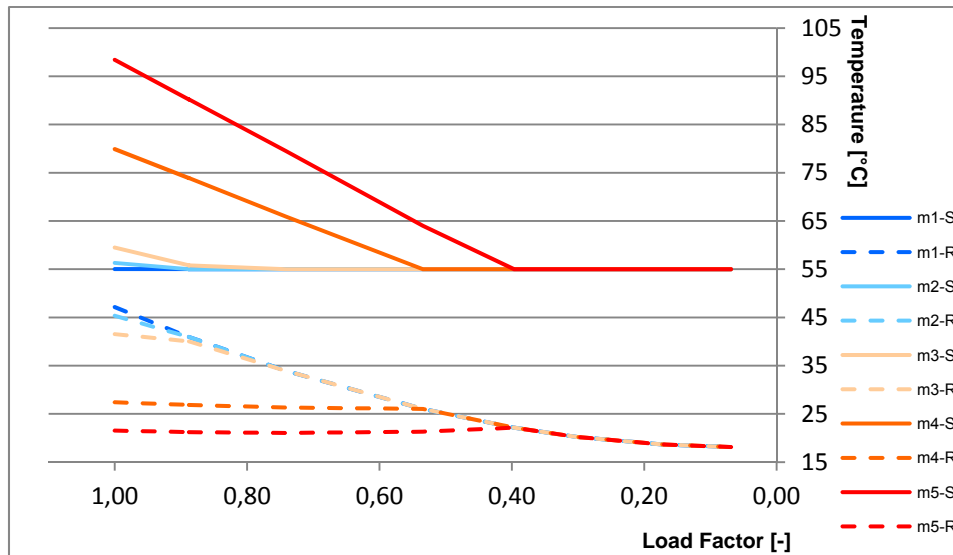
Fig. 1. The supply and return temperature profiles obtained in each mass flow limit, for the current heat demand situation
