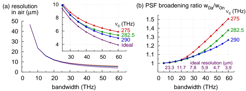
Fig. 4. (a) Calculated values for the axial resolution in air depending on the bandwidth at different center frequencies compared to the ideal reference case without water absorption. (b) The corresponding relative broadening ratios.
