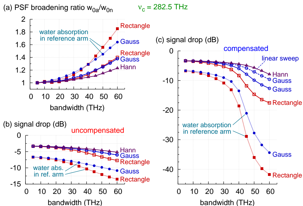
Fig. 7. (a) Relative broadening of the point spread function and (b, c) drop of the amplitude as a function of the bandwidth for different operating parameters with and without compensation for the broadening.
