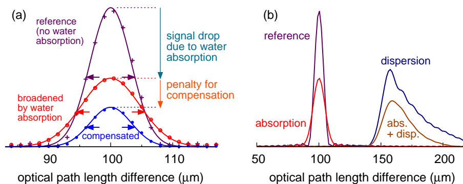
Fig. 2. Point spread functions (PSFs) calculated using a 1/e^2 -truncated Gaussian spectrum centered at 280 THz ( \sim 1071 nm) with 60 THz total width ( \sim 232 nm). (a) Key figures of the numerical investigation: PSF broadening and amplitude drop due to the water absorption compared to reference PSF, and additional amplitude drop due to compensation of the broadening by spectral shaping. Data points: calculated values; curves: fitted Gaussian. (b) Comparison of the broadening effects of absorption and dispersion. Refractive index data by Schiebener et al. [35].
