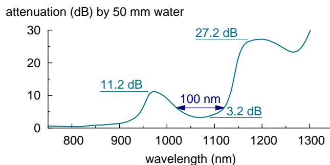
Fig. 1. In addition to the wavelength range below 950 nm, there is a minimum of the water absorption around 1060 nm, that permits in vivo OCT imaging of the human retina. For a length of 50 mm water—corresponding to a double pass through a human eye—this window has a 3 dB-width of approximately 100 nm. Calculated from data by Palmer and Williams [30].
