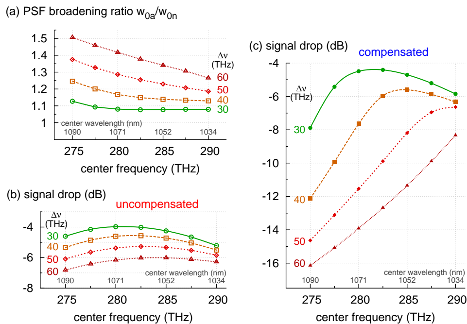
Fig. 6. (a) Relative broadening of the point spread function and (b, c) drop of the amplitude as a function of the center frequency for different bandwidths with and without compensation for the broadening.
