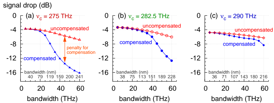
Fig. 5. Drop of the point spread function amplitude due to water absorption as a function of the bandwidth at different center frequencies with and without compensation for the broadening.
