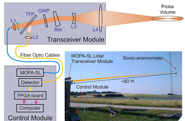
Fig. 1. (Color online) Schematic of a deployable SL-based homodyne cw lidar consisting of transceiver (15 cm × 15 cm × 45 cm) and control (50 cm × 30 cm × 75 cm) modules linked by two fiber optic cables. The “all-optical” transceiver is composed of collimating lens L1, thin-film polarizer (TFP), \lambda/4 wave plate (QWP), reference wedge (RW) for generating a local oscillator beam, telescope lenses L3 and L4, and coupling lens L2. All sensitive electronics are part of the control module. The inset shows a photo of the field test to compare the performance of our lidar wind sensor against a three-dimensional sonic anemometer (F2901 Metek, Germany).
