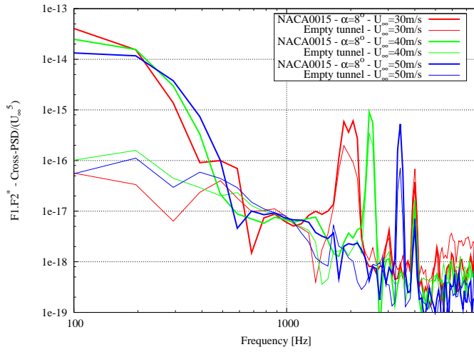
(b) Normalized Cross-PSD (Spectrum normalized by U_\infty^5 )
