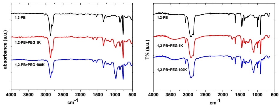
Figure 7.5 IR spectra of ATR mode (left) and transmission mode (right) for nanoporous membranes before and after static adsorption of PEG1K and PEG100K.
