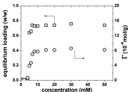
Figure 8.6 Equilibrium loading (squares) of SDS aqueous solution and the final SDS adsorption (circles) in nanoporous 1,2-PB films at different initial bulk concentrations.
