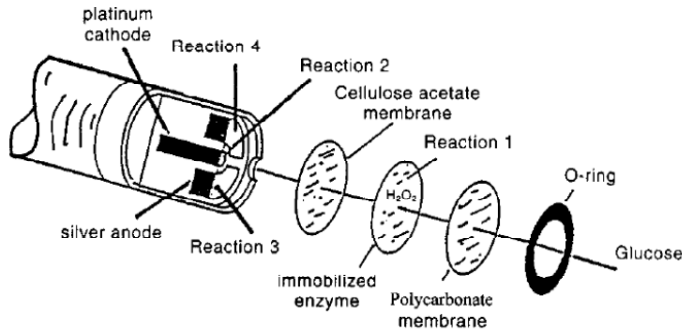
Figure 2.4 Schematic drawing of a ‘first-generation’ glucose biosensor (based on a probe manufactured by YSI Inc.). 51
