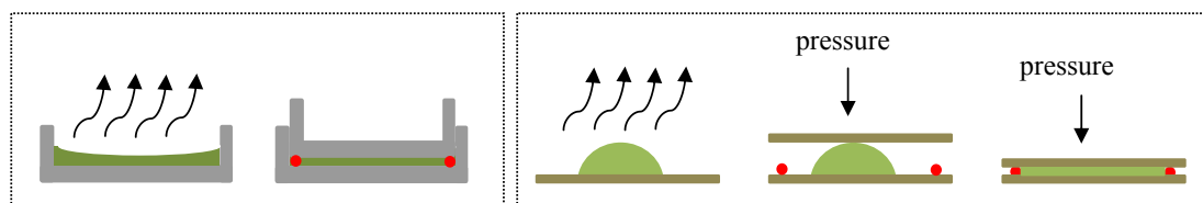
Figure 3.2 Schematic illustration of solvent casting of the precursor solutions (green) onto a petri-dish (grey) for preparation of thick membranes (left) and onto a flat plate (glass or FTDS-coated glass, dark yellow) for preparation of thin membranes (right). Spacers (red) with a desired thickness were used for membrane thickness control.
