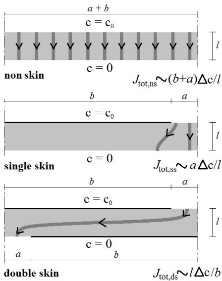
Figure 6.8 Proposed models exhibiting the type of diffusive transport observed for the ns, ss and ds membranes. The membranes are modeled as sheets of thickness l (grey areas) and the skin layer as an infinitely thin impermeable film (black lines) with defects. Defects are presented as parallel non skin stripes of width 2a and regular spacing 2(b+a) . Cross-sections of only the symmetry units of the model are shown. In the case of double skin membrane the bottom skin layer is modeled with cracks parallel to those on the upper surface displaced by a+b . The dark grey lines with arrows schematically show diffusion transport lines for glucose. The concentrations at t=0 are shown. The approximate relations for total fluxes are expected to be valid at the limiting case of l/b \ll 1 and a/b \ll 1 .
