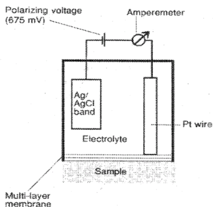
Figure 6.2 A diagram of the electrode chain in amperometric measurements, consisting of the sample, the two electrodes (Pt anode and Ag cathode) and the reference AgCl band, an amperemeter, a voltage source, the membranes and the electrode solutions. 2
