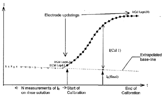
Figure 6.6 A schematic illustration of the registration of electrode response vs. time in expression of upd .
