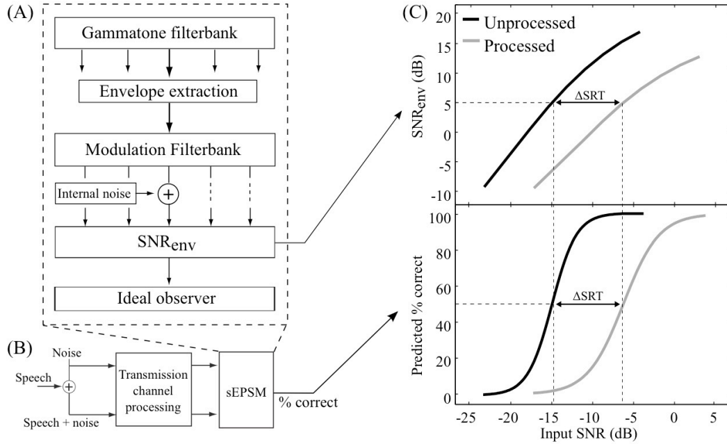
Fig. 1: (A) Block-diagram of the sEPSM processing structure. (B) Scheme for predicting speech intelligibility using the sEPSM. (C) \text{SNR}_{\text{env}} as a function of the input SNR (top panel) and the corresponding predicted percentage of correct responses (bottom panel).
