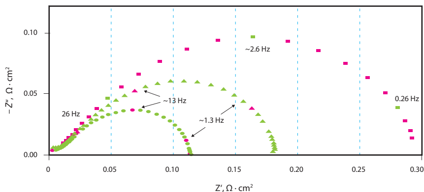
Fig. 4.7. Electrochemical impedance spectroscopy plot of simple composite electrodes of (\text{La}_{0.6}\text{Sr}_{0.4})_{0.99}\text{CoO}_3 and \text{Ce}_{0.9}\text{Gd}_{0.1}\text{O}_{1.95} (■) and the same electrodes impregnated with nanoparticles of \text{Ce}_{0.9}\text{Sm}_{0.1}\text{O}_{1.95} (△) and \text{CeO}_2 (○) at 600°C and zero current in air. The especially surprising aspect is the great improvement: the decrease in electrode polarization resistance ( Z' ), by nanoparticles of pure ceria ( \text{CeO}_2 ), because pure ceria is not supposed to have any electron or ion conductivity in air. The interpretation is that the nanoparticles change the surface chemistry of (\text{La}_{0.6}\text{Sr}_{0.4})_{0.99}\text{CoO}_3 and \text{Ce}_{0.9}\text{Gd}_{0.1}\text{O}_{1.95} and, through this, accelerate the oxygen electrode reaction.
