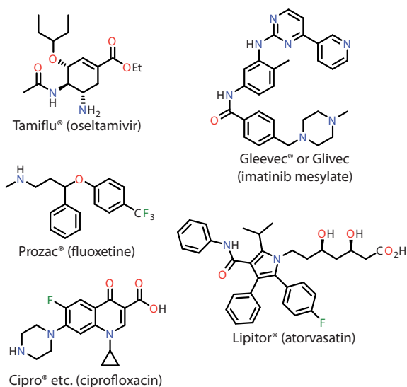
Fig. 19.1. Synthetic small molecules with diverse, bio-medically important properties produced by major pharmaceutical companies. Gleevec® or Glivec® (imatinib mesylate, Novartis) is used to treat a blood cancer called chronic myeloid leukemia. Cipro® and other trade names (ciprofloxacin, Bayer and other manufacturers) has broad-spectrum antibiotic activities. Tamiflu® (oseltamivir, Roche) displays antiviral activity against influenza viruses. Lipitor® (atorvastatin, Pfizer) is used to lower serum cholesterol and the risk of heart disease. Prozac® (fluoxetine, Eli Lilly and other manufacturers) is an antidepressant used for mood disorders.
