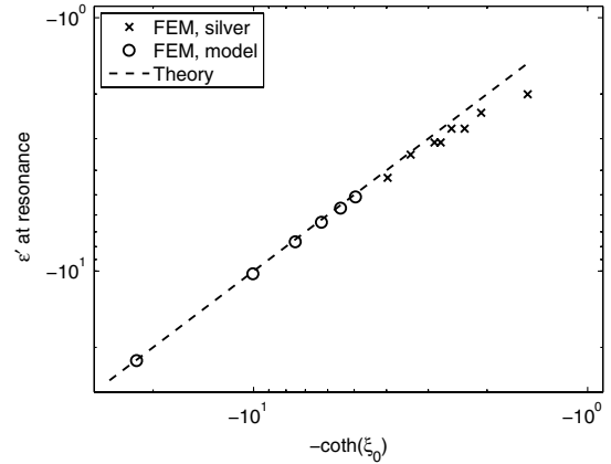
Fig. 3. Value of real part of permittivity \epsilon as a function of affinity of the cylinders for main resonance, n = 1 . It was taken a = 50 nm, \epsilon'' = 0.6 , and \lambda = 2 \mu\text{m} in numerical simulations for model metal. For silver, a = 15 nm was taken.
