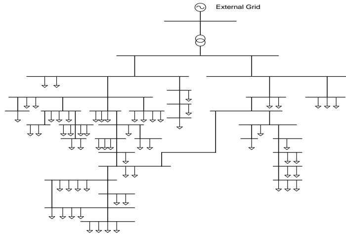
Figure 2 Bornholm 400 V Grid Model in PowerFactory
