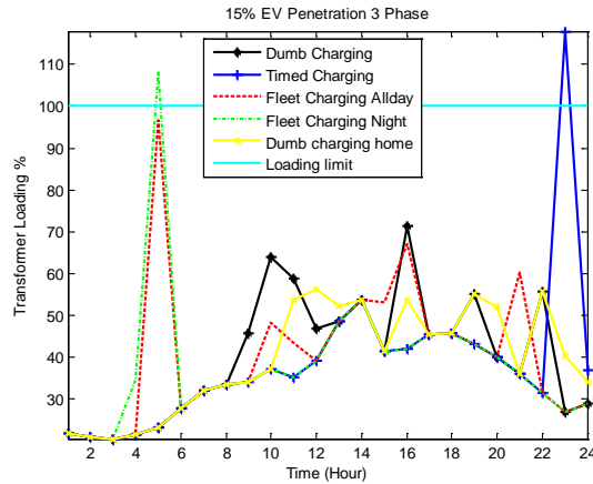
Figure 5 Transformer loading 400 V – 15% EV penetration and 3 phase charging
