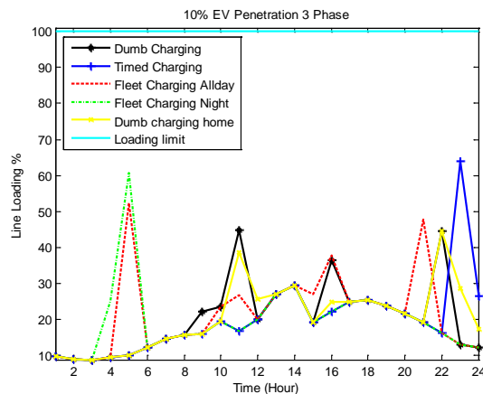
Figure 3 Line Loading 400 V – 10% EV penetration and 3 phase charging
