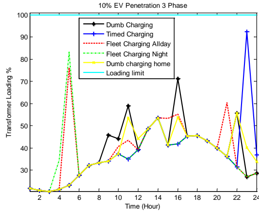
Figure 4 Transformer loading 400 V – 10% EV penetration and 3 phase charging
