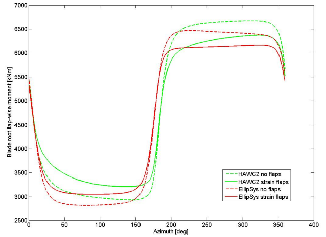
Figure 15 – Blade root flap-wise bending moment for the NREL 5MW reference turbine operating in half-wake with and without the feedback flap control based on blade root flap-wise bending moment.
