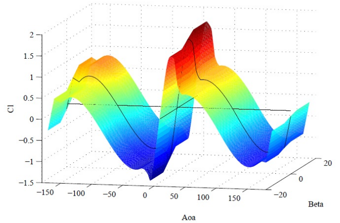
Figure 7 - Lift coefficient C_L^{st} in the case of an airfoil with trailing edge flap. The lift is a function of both angle of attack \alpha and flap deflection \beta , and is represented by a surface in space.
