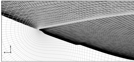
Figure 2 - 3D surface mesh around the NREL 5MW reference turbine blade.
