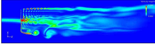
Figure 22 – Top view of the NREL 5MW reference turbine operating in half-wake with the prescribed flap control showing contours of vorticity magnitude in a horizontal plane through the rotor center – \pm 5 deg flap.
