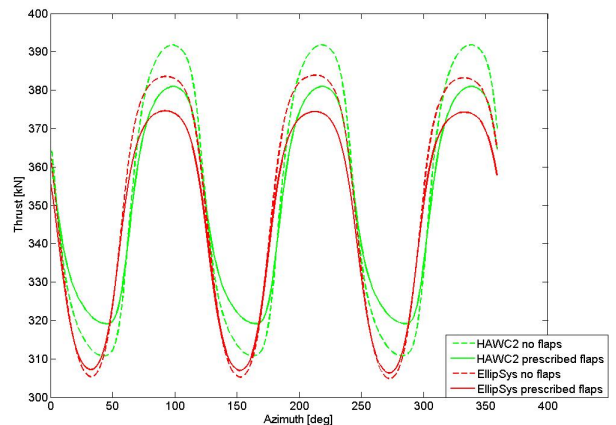
Figure 9 - Rotor thrust for the NREL 5MW reference turbine operating in half-wake with and without the prescribed flap control.
