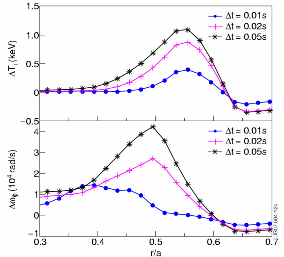
Figure 7. As in figure 6, but for simulated (a) \Delta T_i and (b) \Delta\omega_\phi profiles with a model of v_{\text{pinch}}\approx -15 m/s and P_r=1.0 .
