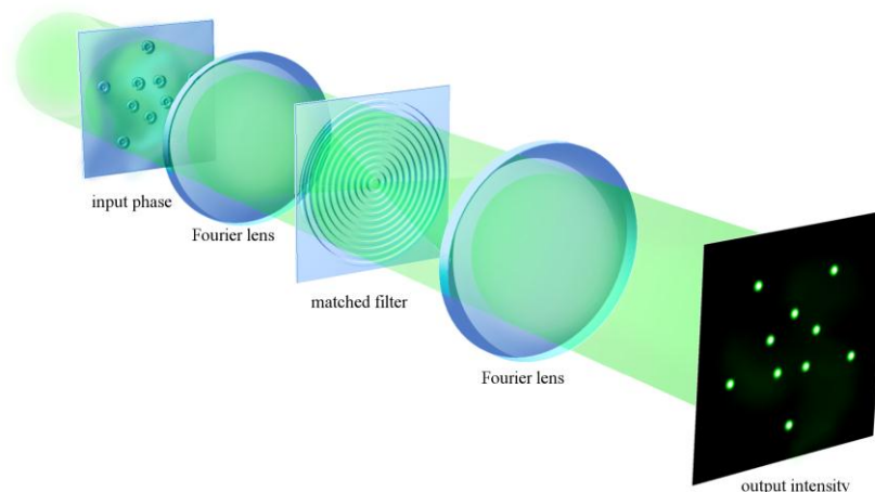
Fig. 1. The matched-filtering Generalized Phase Contrast (mGPC) setup. High intensity spots corresponding to desired correlation target patterns are generated at the output despite mild phase distortions at the input phase.
