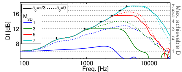
Figure 4 - Directivity index for elevated and horizontal beams
