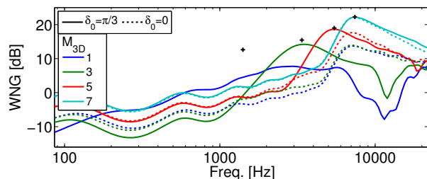
Figure 3 - White noise gain for a horizontal (dashed) and vertical (solid) beam
