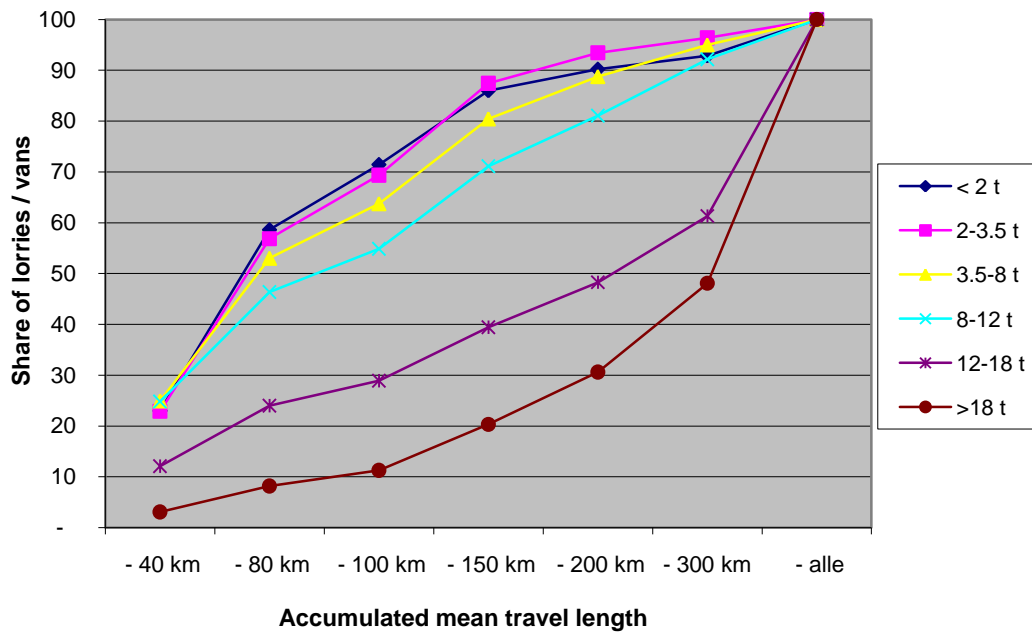
Figure 4 Accumulated distribution of the mean travel length of vans and lorries when it is assumed that they drive 225 working days per year. Source: MD database
