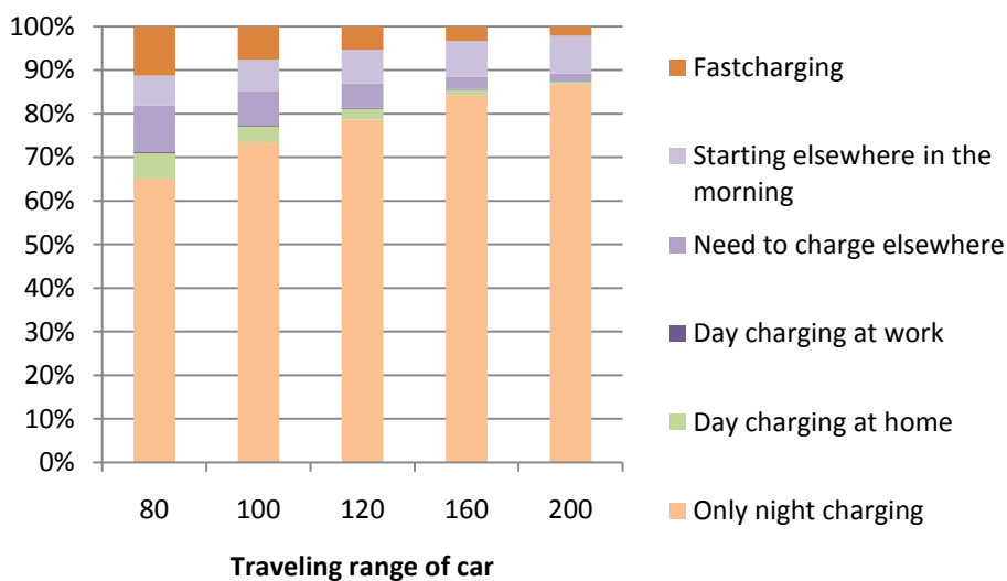
Figure 5 The share of driving cars that will do with night charging at home and the share that need to charge during the day in different ways. Source: Akta data
