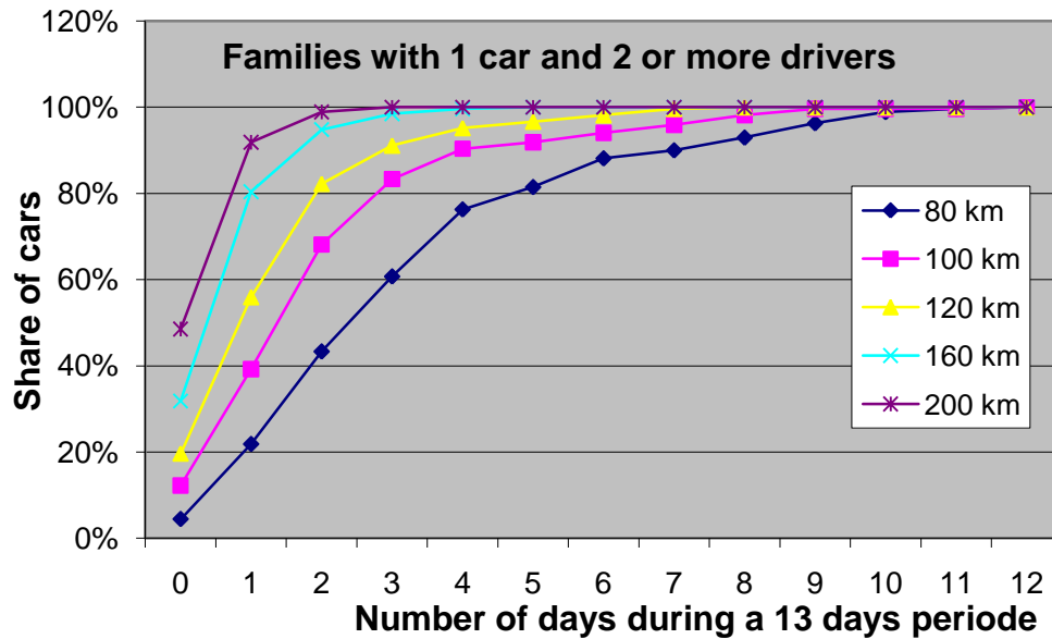
Figure 2 Share of cars needing to be charged away from home 0, 1, 2 etc. days during a 13 days period. Represents a family with one car and 2 or more driving licences in Greater Copenhagen. Akta data
