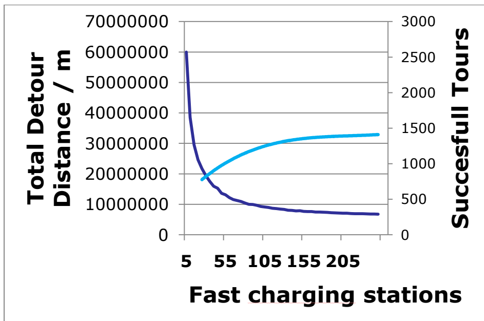
Figure 9 Total detour in meter depending of the number of fast charging stations, left axes. The number of tours which gets fast charging (1441 tours in all), right axes.
