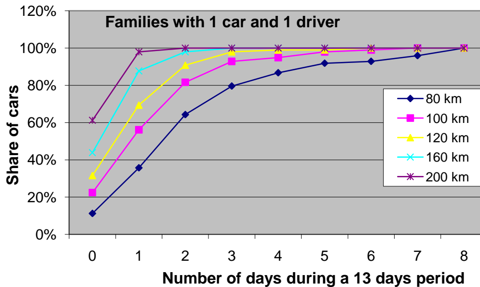
Figure 3 Share of cars needing to be charged away from home 0, 1, 2 etc. days during a 13 days period. Represents singles in Greater Copenhagen. Akta data
