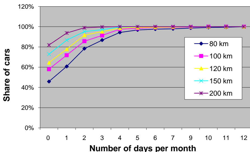
Figure 7 Share of cars that needs to perform fast charging within a month, on only a few or several days. Source: Akta data
