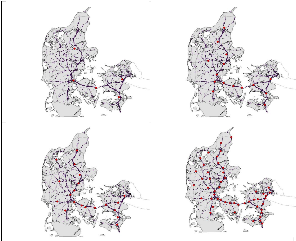
Figure 8 Localisation of 5,15, 20 and 50 fast charging stations calculated by the model. The black spots shows the Fast Charge potential Points from the trips
