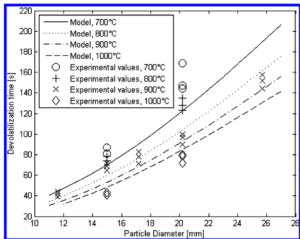
Figure 13. Comparison of pine wood devolatilization time predicted by the model and by experimentally found values. 10% O 2 , 5% volumetric fill degree in kiln. Y = 0.2. α = 1.9 · 10 -7 m 2 /s.
